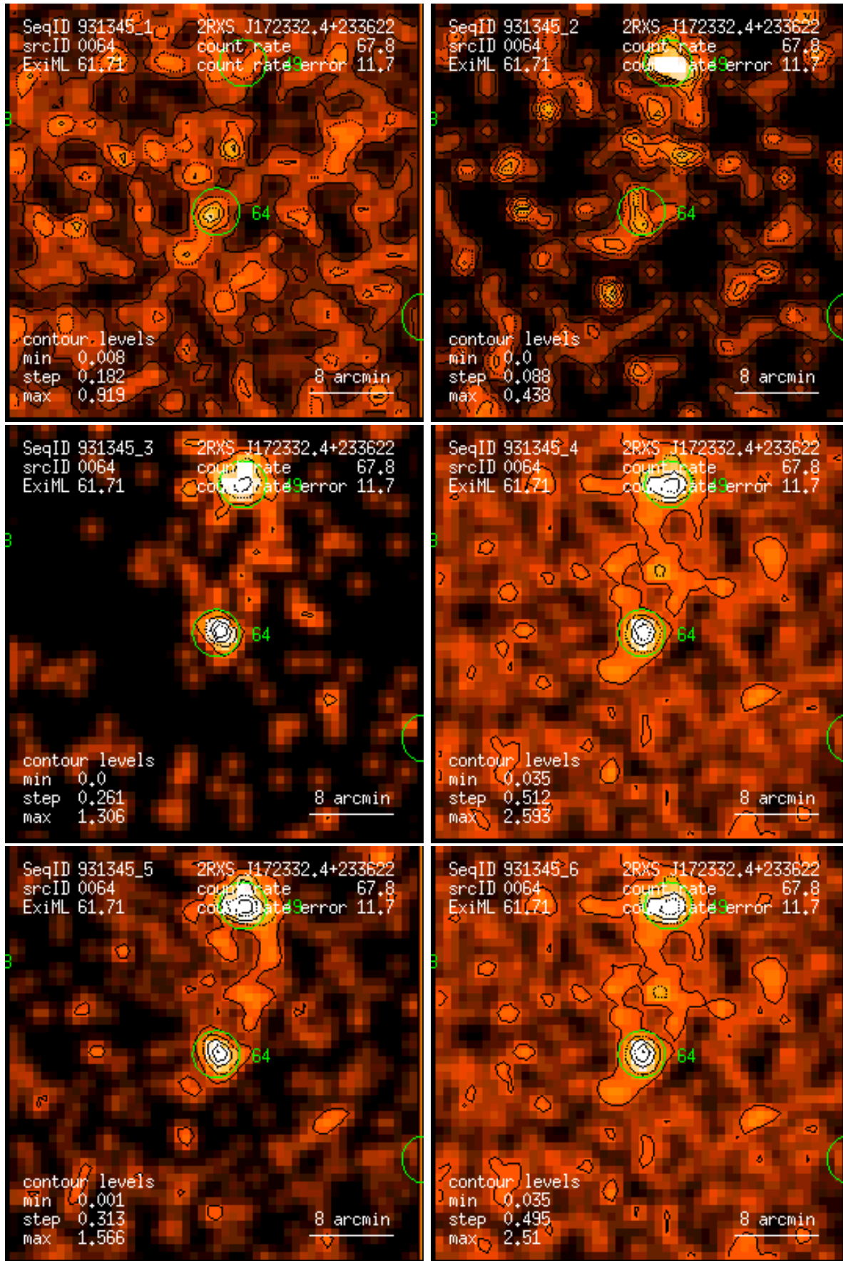
Figure 64: RASS 931345: detection 0064: band rate images, Gaussian filter: (1) PSPC channels 11 – 41, (2) 52 – 90, (3) 91 – 201, (4) 11 – 235, (5) 52 – 201, (6) 11 – 201. Broad band rates in counts/ks. Band rate contour levels in counts/ks/arcmin 2 .
