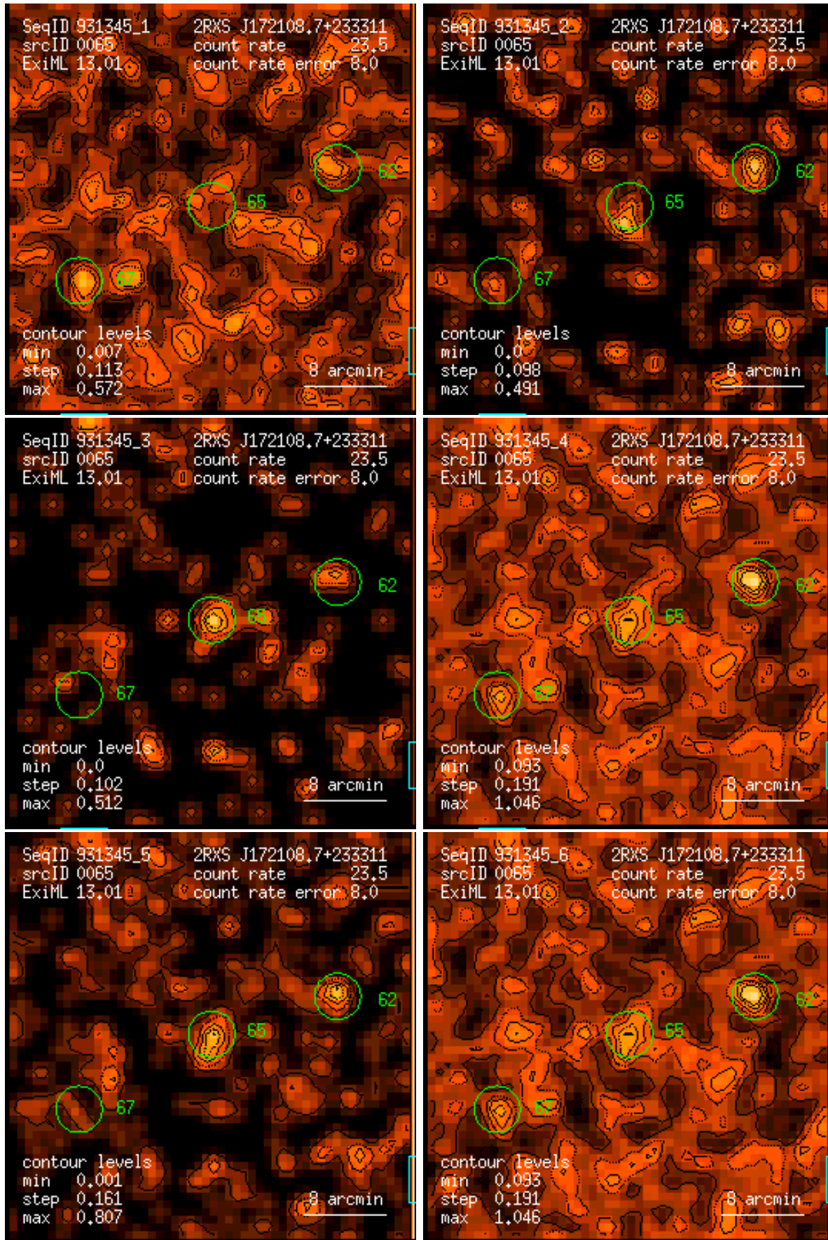
Figure 65: RASS 931345: detection 0065: band rate images, Gaussian filter: (1) PSPC channels 11 – 41, (2) 52 – 90, (3) 91 – 201, (4) 11 – 235, (5) 52 – 201, (6) 11 – 201. Broad band rates in counts/ks. Band rate contour levels in counts/ks/arcmin 2 .
