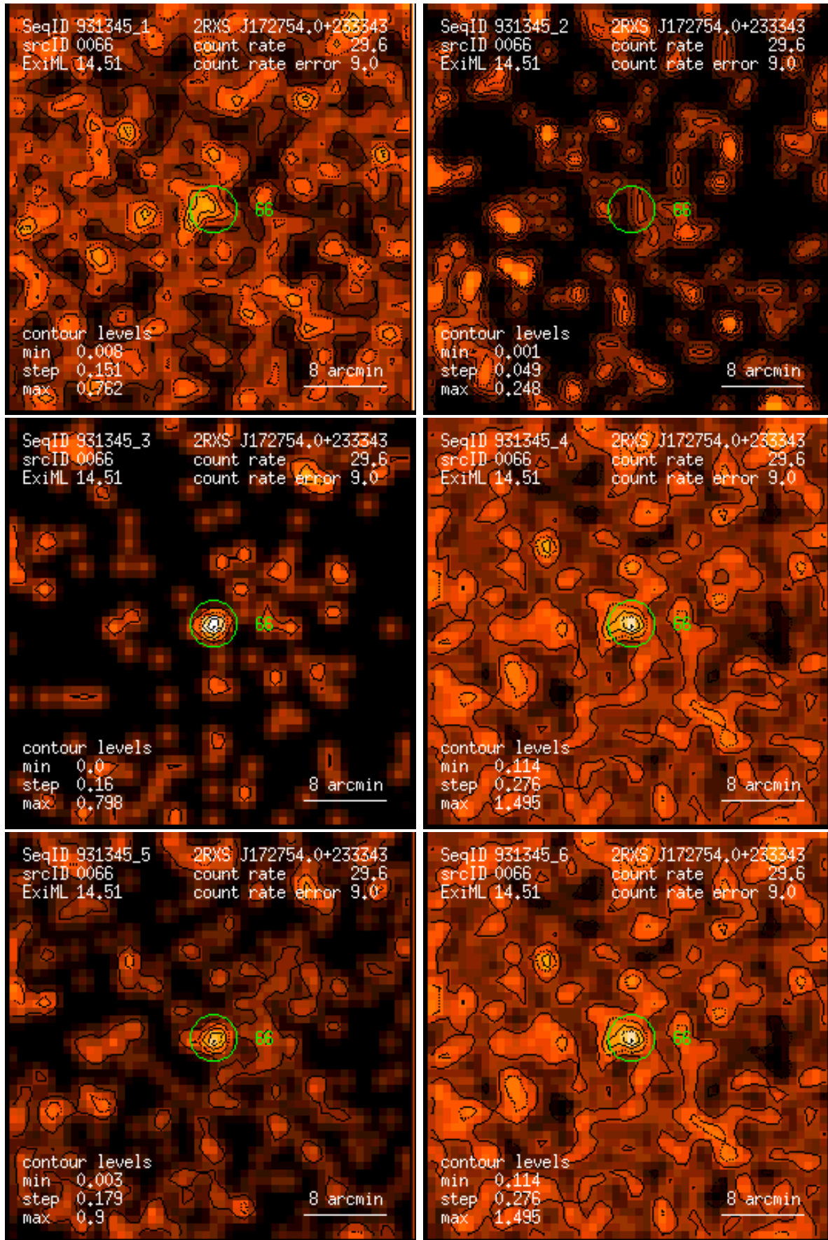
Figure 66: RASS 931345: detection 0066: band rate images, Gaussian filter: (1) PSPC channels 11 – 41, (2) 52 – 90, (3) 91 – 201, (4) 11 – 235, (5) 52 – 201, (6) 11 – 201. Broad band rates in counts/ks. Band rate contour levels in counts/ks/arcmin 2 .
