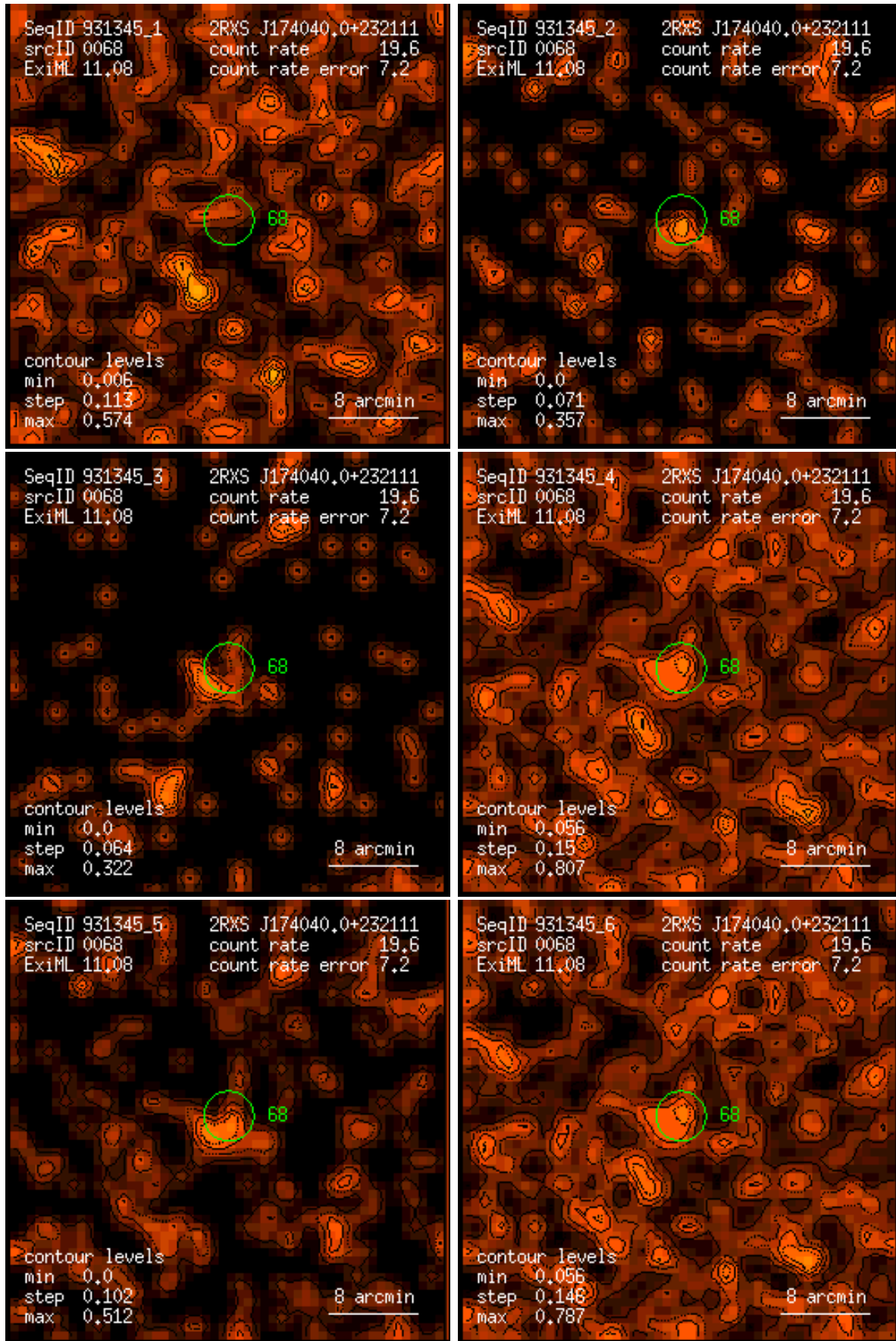
Figure 68: RASS 931345: detection 0068: band rate images, Gaussian filter: (1) PSPC channels 11 – 41, (2) 52 – 90, (3) 91 – 201, (4) 11 – 235, (5) 52 – 201, (6) 11 – 201. Broad band rates in counts/ks. Band rate contour levels in counts/ks/arcmin 2 .
