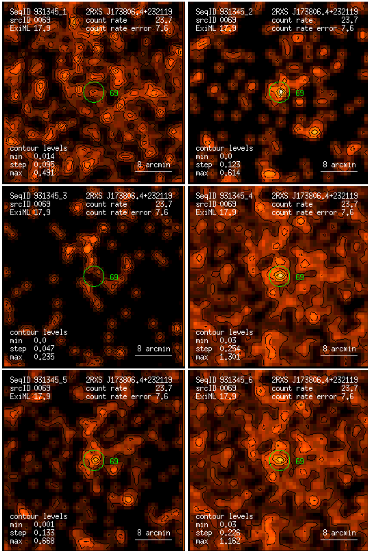
Figure 69: RASS 931345: detection 0069: band rate images, Gaussian filter: (1) PSPC channels 11 – 41, (2) 52 – 90, (3) 91 – 201, (4) 11 – 235, (5) 52 – 201, (6) 11 – 201. Broad band rates in counts/ks. Band rate contour levels in counts/ks/arcmin 2 .
