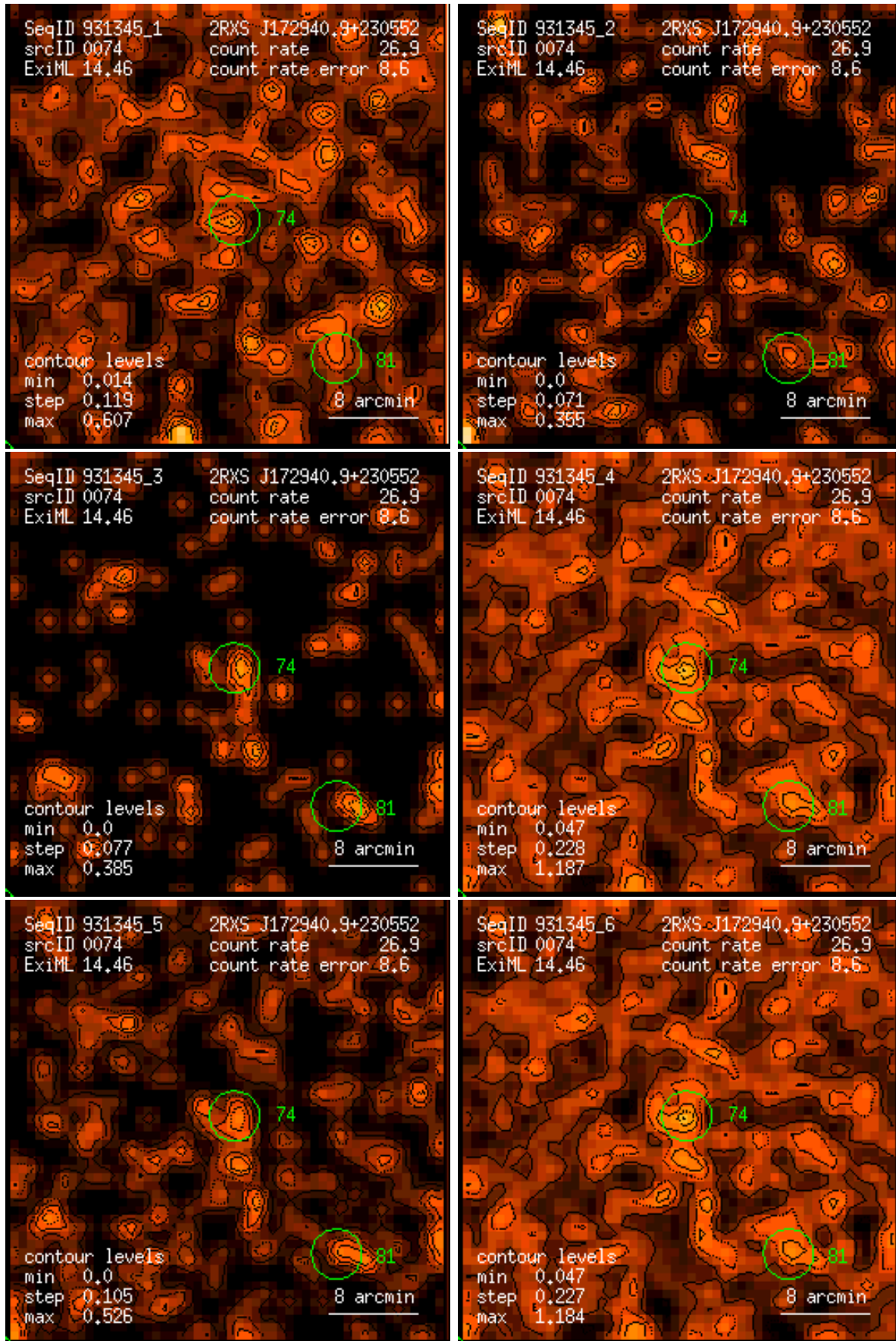
Figure 74: RASS 931345: detection 0074: band rate images, Gaussian filter: (1) PSPC channels 11 – 41, (2) 52 – 90, (3) 91 – 201, (4) 11 – 235, (5) 52 – 201, (6) 11 – 201. Broad band rates in counts/ks. Band rate contour levels in counts/ks/arcmin 2 .
