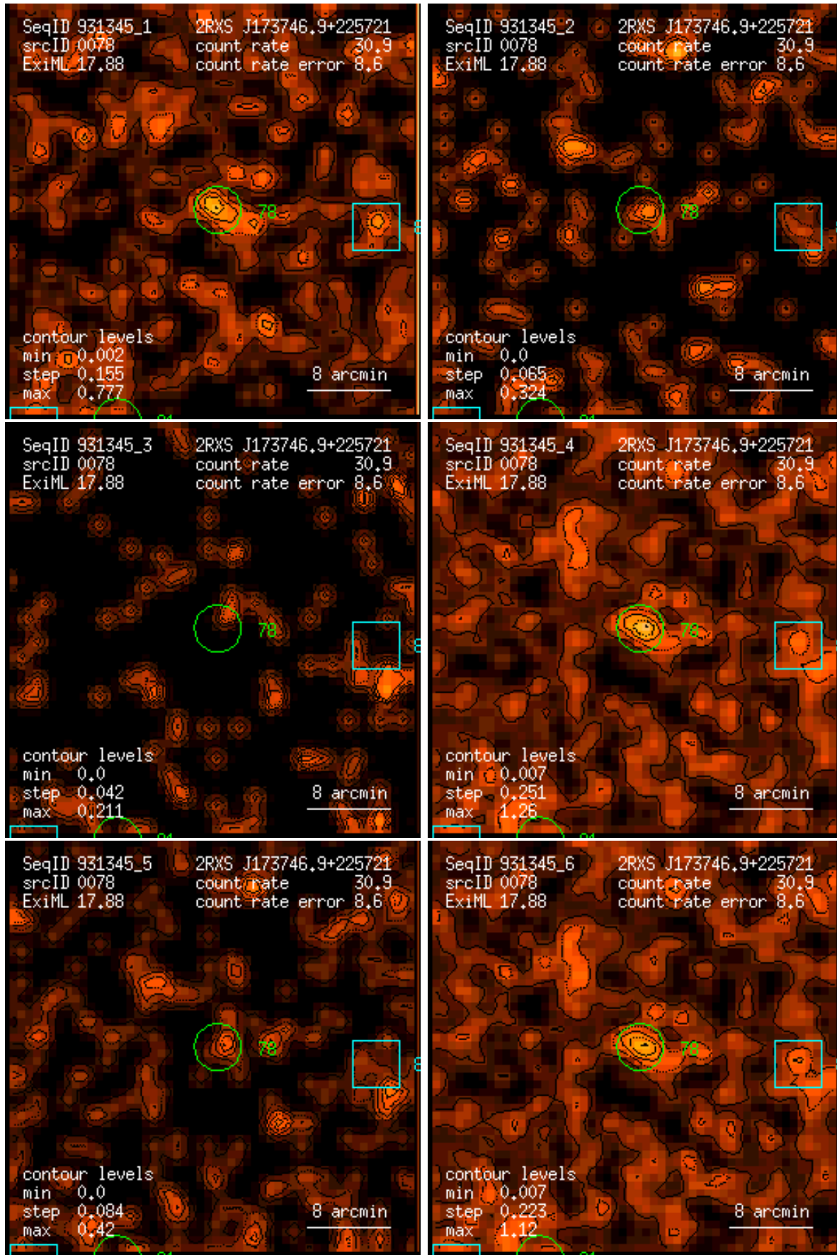
Figure 78: RASS 931345: detection 0078: band rate images, Gaussian filter: (1) PSPC channels 11 – 41, (2) 52 – 90, (3) 91 – 201, (4) 11 – 235, (5) 52 – 201, (6) 11 – 201. Broad band rates in counts/ks. Band rate contour levels in counts/ks/arcmin 2 .
