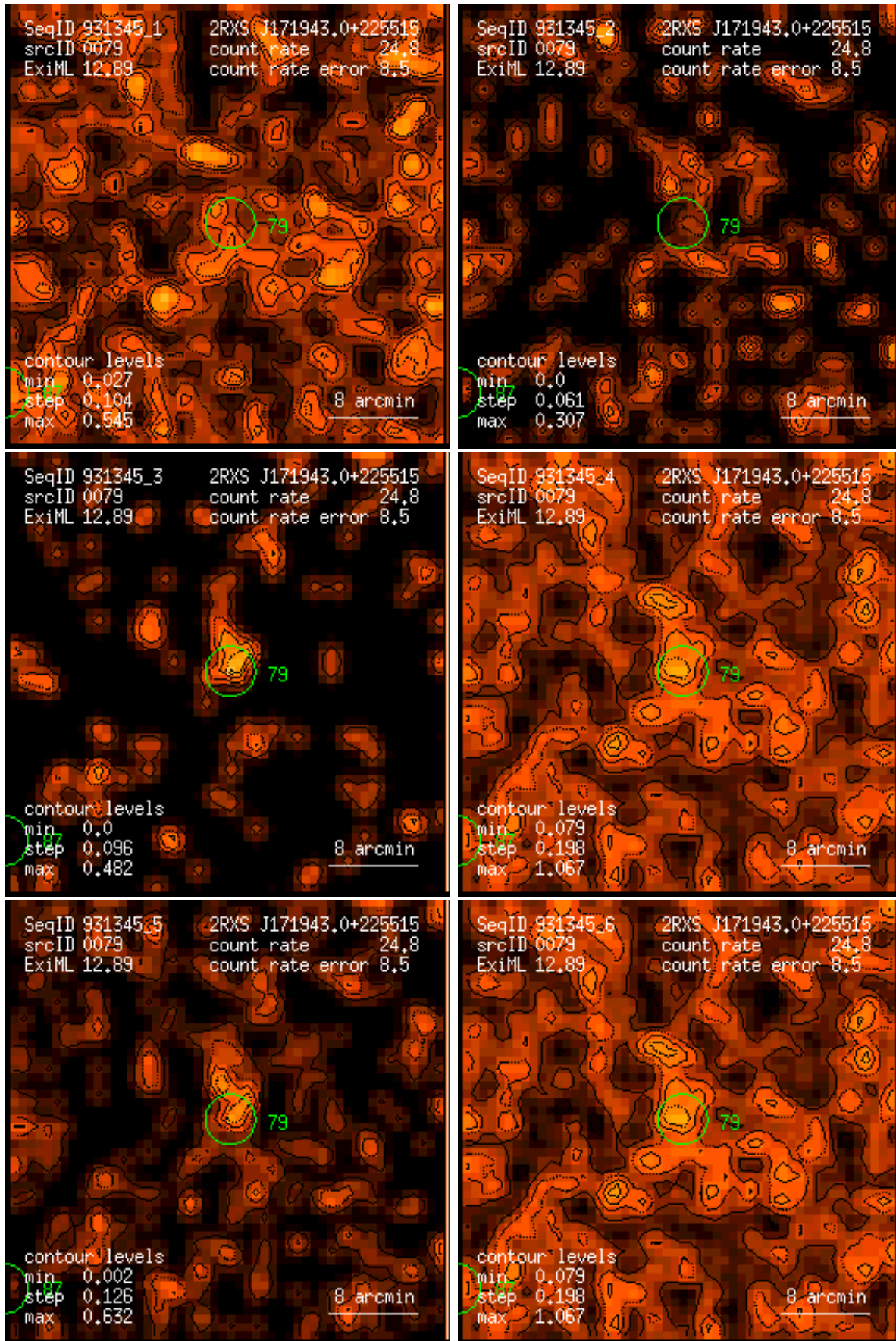
Figure 79: RASS 931345: detection 0079: band rate images, Gaussian filter: (1) PSPC channels 11 – 41, (2) 52 – 90, (3) 91 – 201, (4) 11 – 235, (5) 52 – 201, (6) 11 – 201. Broad band rates in counts/ks. Band rate contour levels in counts/ks/arcmin 2 .
