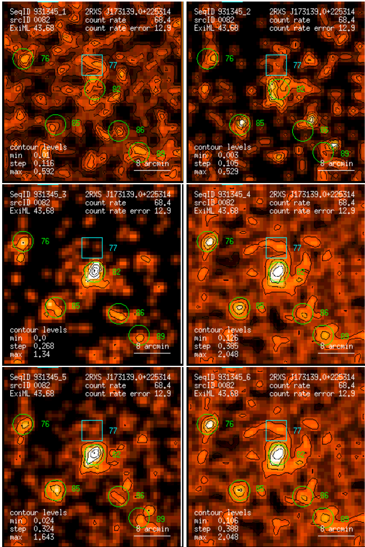
Figure 82: RASS 931345: detection 0082: band rate images, Gaussian filter: (1) PSPC channels 11 – 41, (2) 52 – 90, (3) 91 – 201, (4) 11 – 235, (5) 52 – 201, (6) 11 – 201. Broad band rates in counts/ks. Band rate contour levels in counts/ks/arcmin 2 .
