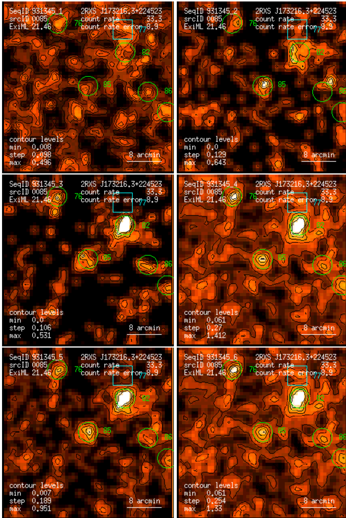
Figure 85: RASS 931345: detection 0085: band rate images, Gaussian filter: (1) PSPC channels 11 – 41, (2) 52 – 90, (3) 91 – 201, (4) 11 – 235, (5) 52 – 201, (6) 11 – 201. Broad band rates in counts/ks. Band rate contour levels in counts/ks/arcmin 2 .
