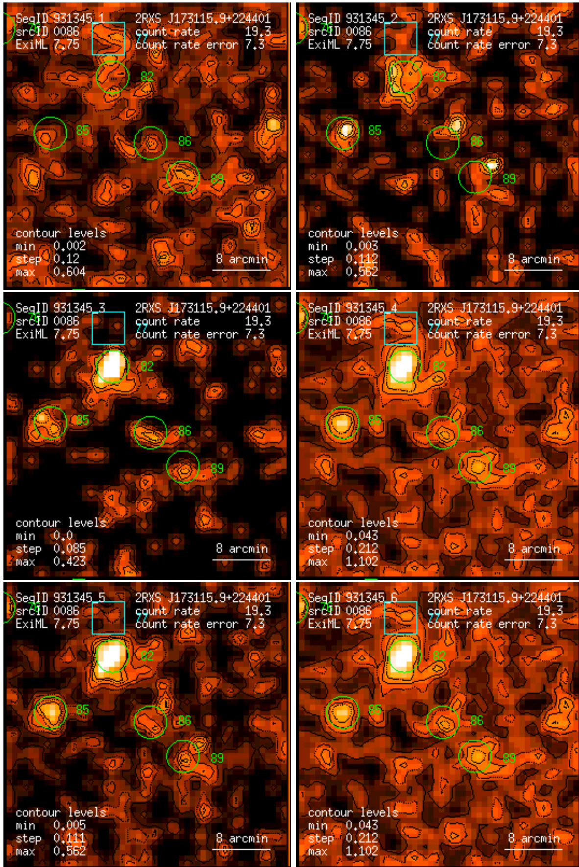
Figure 86: RASS 931345: detection 0086: band rate images, Gaussian filter: (1) PSPC channels 11 – 41, (2) 52 – 90, (3) 91 – 201, (4) 11 – 235, (5) 52 – 201, (6) 11 – 201. Broad band rates in counts/ks. Band rate contour levels in counts/ks/arcmin 2 .
