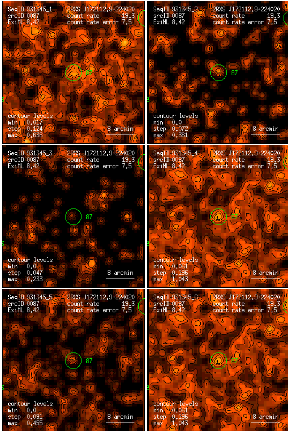
Figure 87: RASS 931345: detection 0087: band rate images, Gaussian filter: (1) PSPC channels 11 – 41, (2) 52 – 90, (3) 91 – 201, (4) 11 – 235, (5) 52 – 201, (6) 11 – 201. Broad band rates in counts/ks. Band rate contour levels in counts/ks/arcmin 2 .
