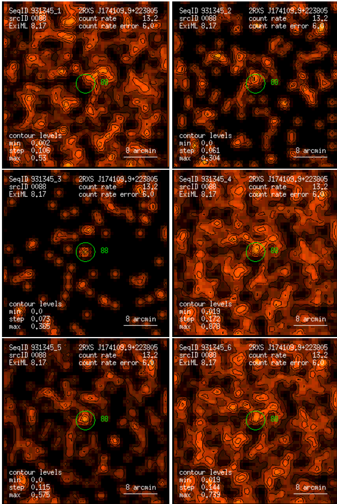
Figure 88: RASS 931345: detection 0088: band rate images, Gaussian filter: (1) PSPC channels 11 – 41, (2) 52 – 90, (3) 91 – 201, (4) 11 – 235, (5) 52 – 201, (6) 11 – 201. Broad band rates in counts/ks. Band rate contour levels in counts/ks/arcmin 2 .
