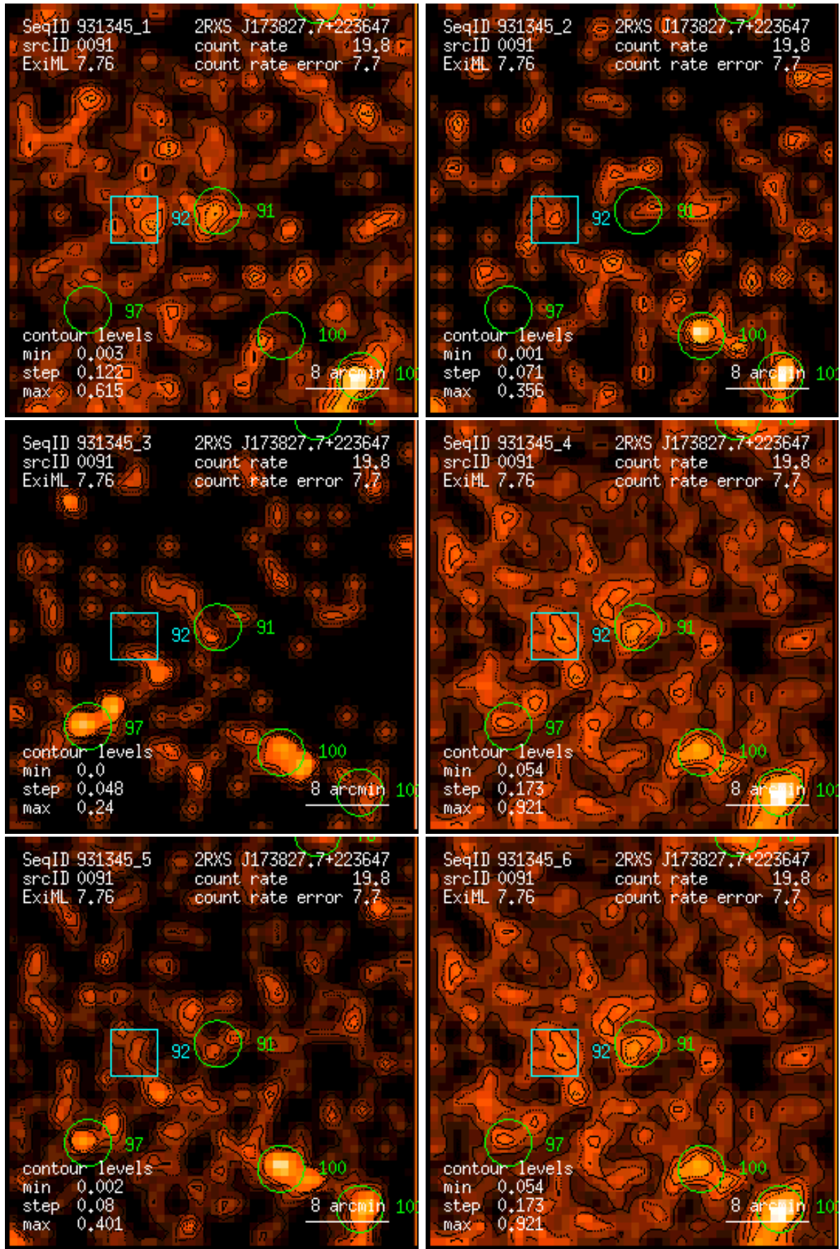
Figure 91: RASS 931345: detection 0091: band rate images, Gaussian filter: (1) PSPC channels 11 – 41, (2) 52 – 90, (3) 91 – 201, (4) 11 – 235, (5) 52 – 201, (6) 11 – 201. Broad band rates in counts/ks. Band rate contour levels in counts/ks/arcmin 2 .
