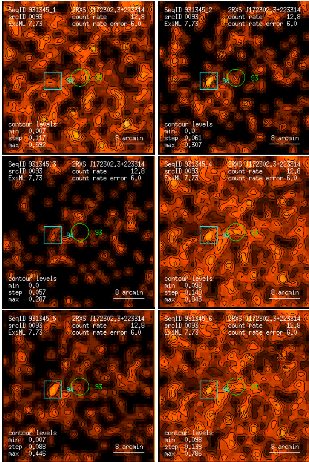
Figure 93: RASS 931345: detection 0093: band rate images, Gaussian filter: (1) PSPC channels 11 – 41, (2) 52 – 90, (3) 91 – 201, (4) 11 – 235, (5) 52 – 201, (6) 11 – 201. Broad band rates in counts/ks. Band rate contour levels in counts/ks/arcmin 2 .
