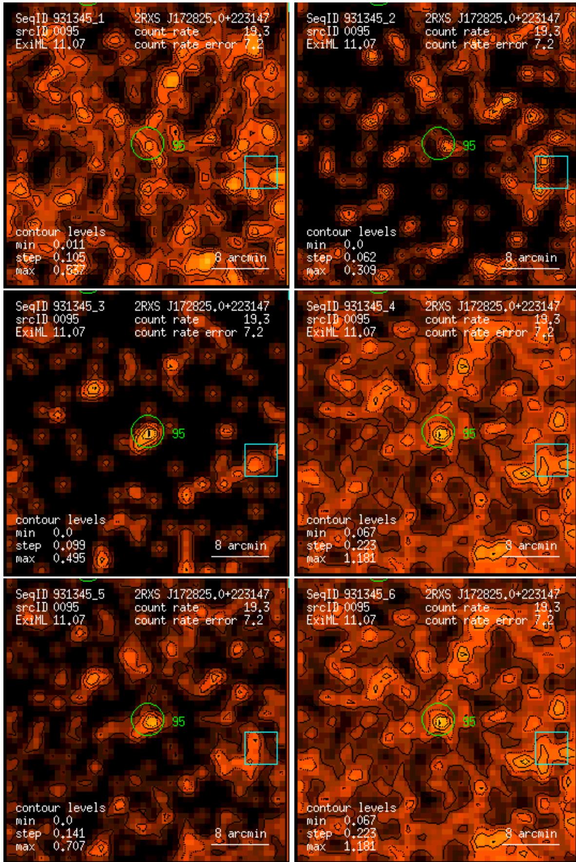
Figure 95: RASS 931345: detection 0095: band rate images, Gaussian filter: (1) PSPC channels 11 – 41, (2) 52 – 90, (3) 91 – 201, (4) 11 – 235, (5) 52 – 201, (6) 11 – 201. Broad band rates in counts/ks. Band rate contour levels in counts/ks/arcmin 2 .
