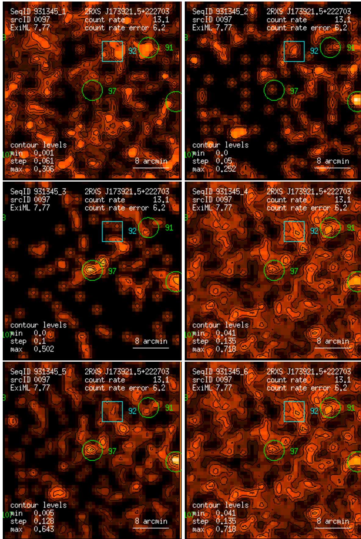
Figure 97: RASS 931345: detection 0097: band rate images, Gaussian filter: (1) PSPC channels 11 – 41, (2) 52 – 90, (3) 91 – 201, (4) 11 – 235, (5) 52 – 201, (6) 11 – 201. Broad band rates in counts/ks. Band rate contour levels in counts/ks/arcmin 2 .
