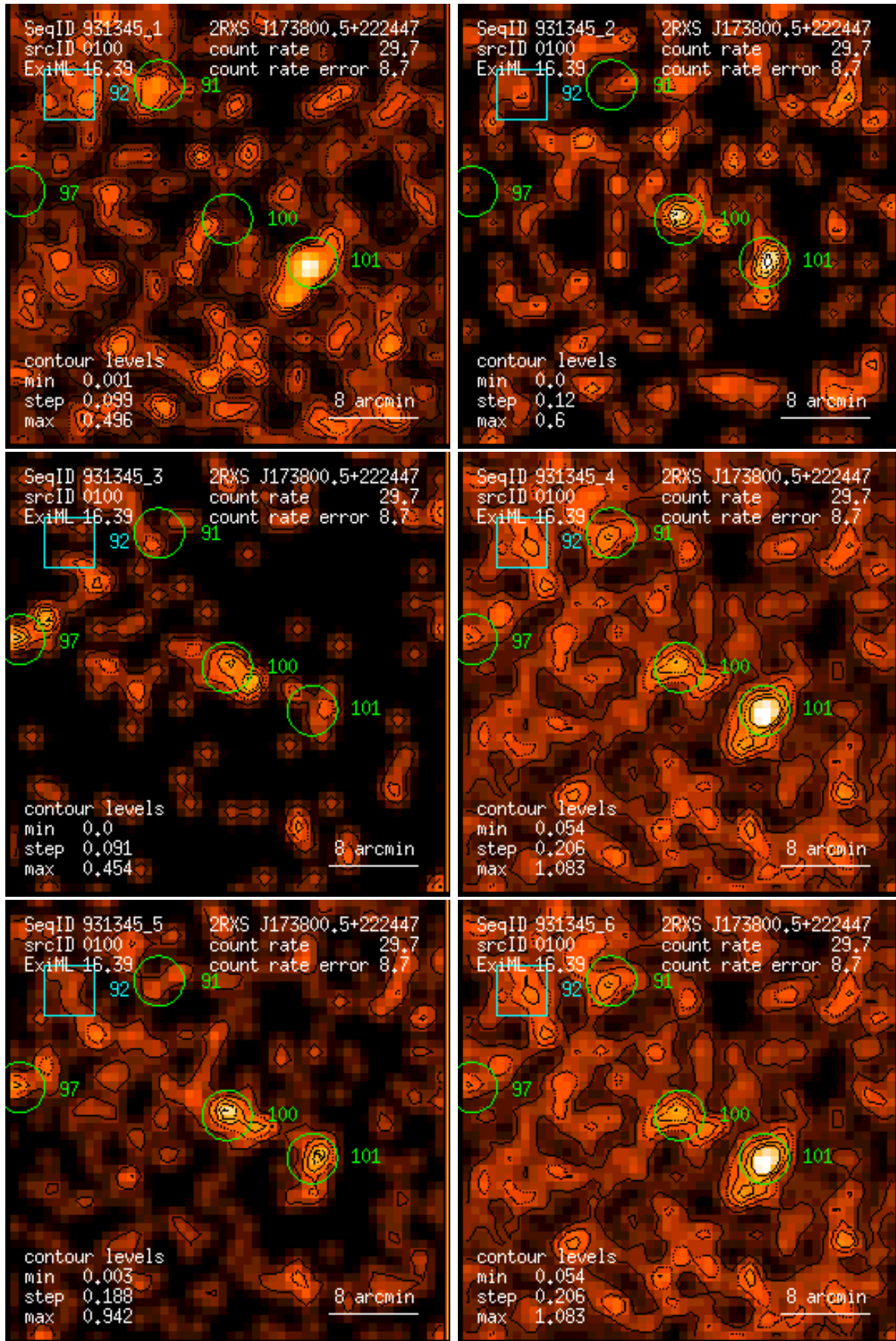
Figure 100: RASS 931345: detection 0100: band rate images, Gaussian filter: (1) PSPC channels 11 – 41, (2) 52 – 90, (3) 91 – 201, (4) 11 – 235, (5) 52 – 201, (6) 11 – 201. Broad band rates in counts/ks. Band rate contour levels in counts/ks/arcmin 2 .
