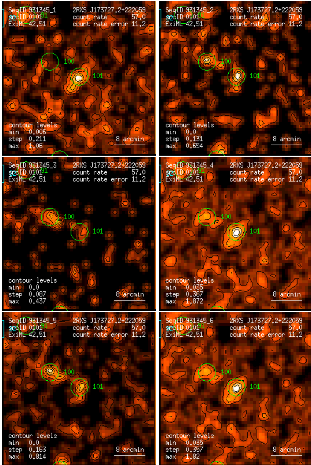
Figure 101: RASS 931345: detection 0101: band rate images, Gaussian filter: (1) PSPC channels 11 – 41, (2) 52 – 90, (3) 91 – 201, (4) 11 – 235, (5) 52 – 201, (6) 11 – 201. Broad band rates in counts/ks. Band rate contour levels in counts/ks/arcmin 2 .
