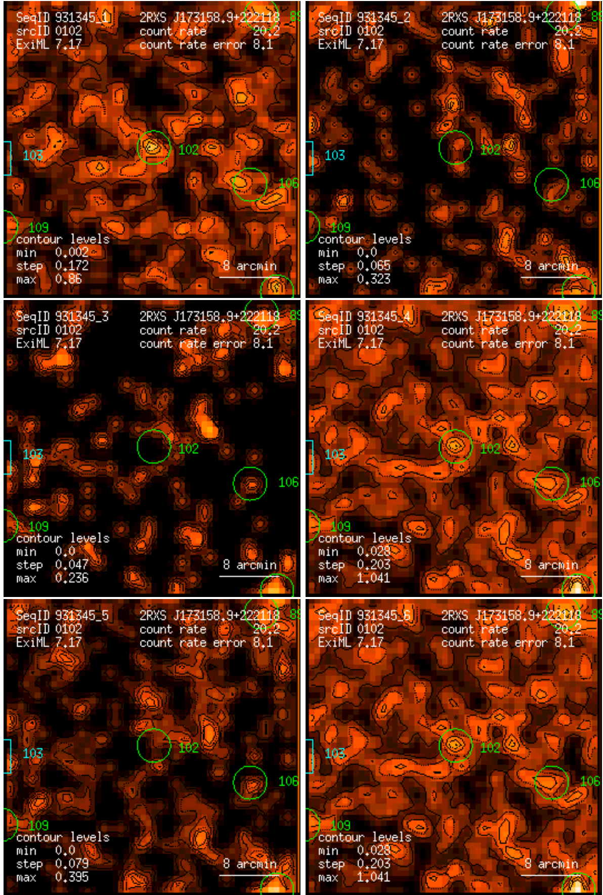
Figure 102: RASS 931345: detection 0102: band rate images, Gaussian filter: (1) PSPC channels 11 – 41, (2) 52 – 90, (3) 91 – 201, (4) 11 – 235, (5) 52 – 201, (6) 11 – 201. Broad band rates in counts/ks. Band rate contour levels in counts/ks/arcmin 2 .
