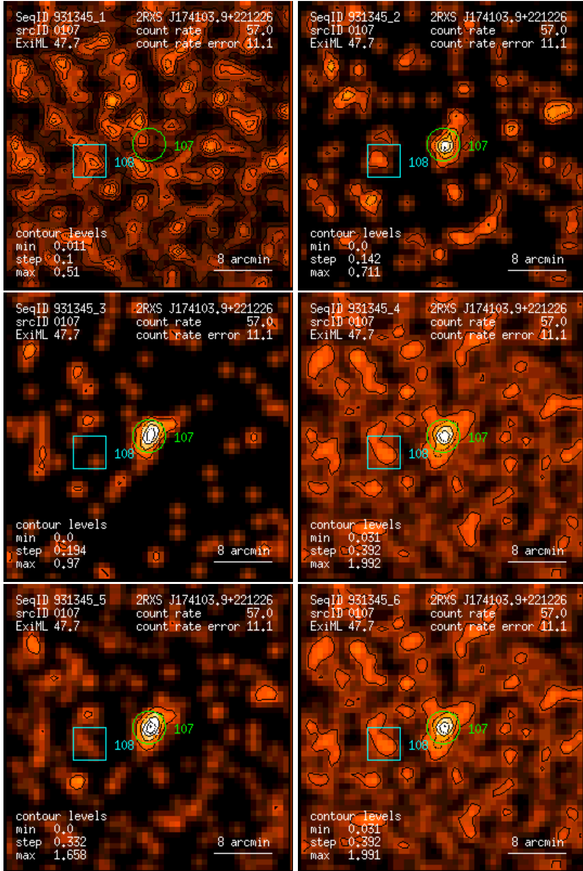
Figure 107: RASS 931345: detection 0107: band rate images, Gaussian filter: (1) PSPC channels 11 – 41, (2) 52 – 90, (3) 91 – 201, (4) 11 – 235, (5) 52 – 201, (6) 11 – 201. Broad band rates in counts/ks. Band rate contour levels in counts/ks/arcmin 2 .
