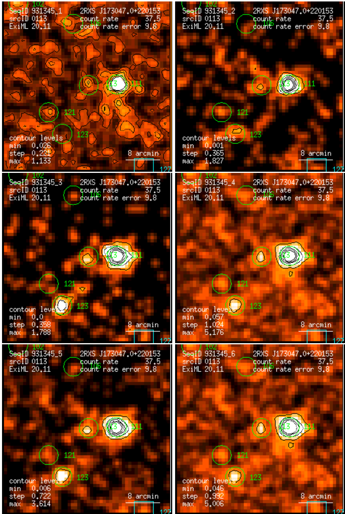
Figure 113: RASS 931345: detection 0113: band rate images, Gaussian filter: (1) PSPC channels 11 – 41, (2) 52 – 90, (3) 91 – 201, (4) 11 – 235, (5) 52 – 201, (6) 11 – 201. Broad band rates in counts/ks. Band rate contour levels in counts/ks/arcmin 2 .
