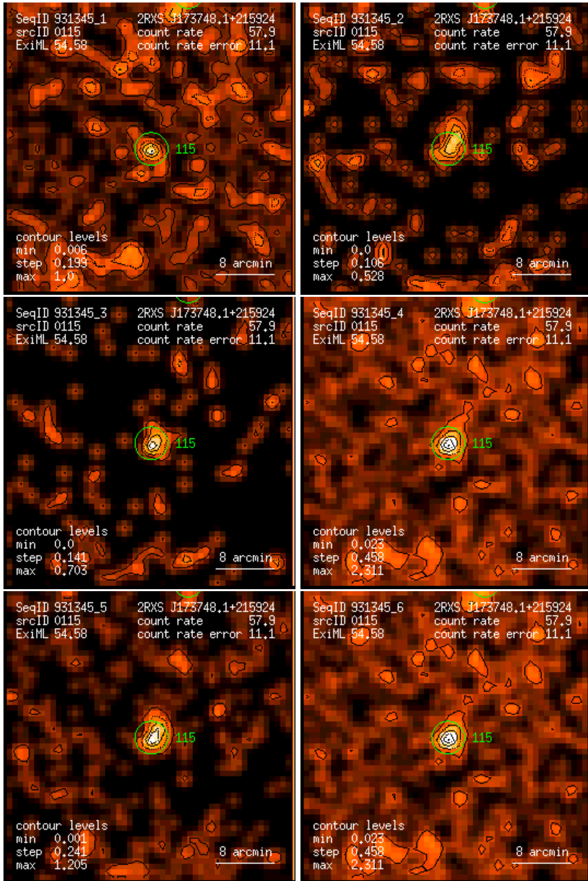
Figure 115: RASS 931345: detection 0115: band rate images, Gaussian filter: (1) PSPC channels 11 – 41, (2) 52 – 90, (3) 91 – 201, (4) 11 – 235, (5) 52 – 201, (6) 11 – 201. Broad band rates in counts/ks. Band rate contour levels in counts/ks/arcmin 2 .
