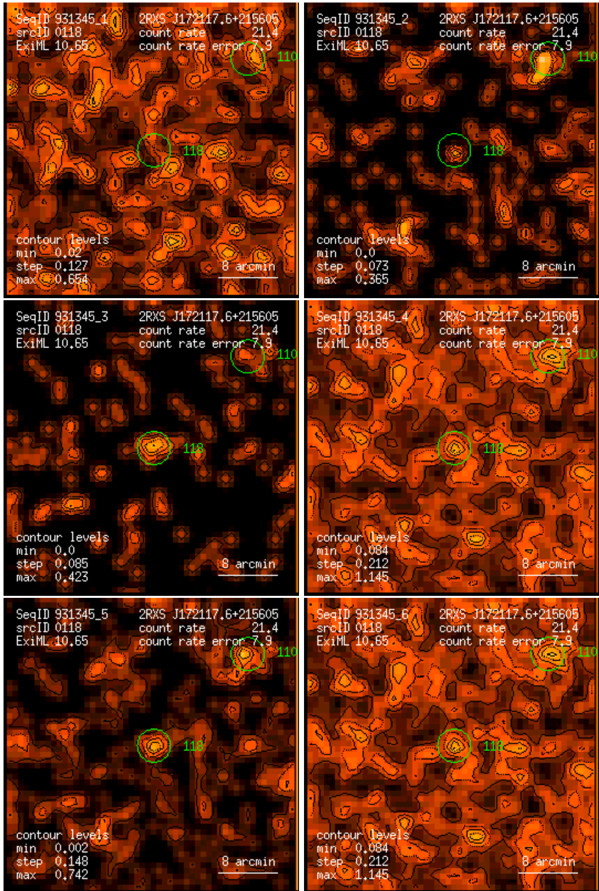
Figure 118: RASS 931345: detection 0118: band rate images, Gaussian filter: (1) PSPC channels 11 – 41, (2) 52 – 90, (3) 91 – 201, (4) 11 – 235, (5) 52 – 201, (6) 11 – 201. Broad band rates in counts/ks. Band rate contour levels in counts/ks/arcmin 2 .
