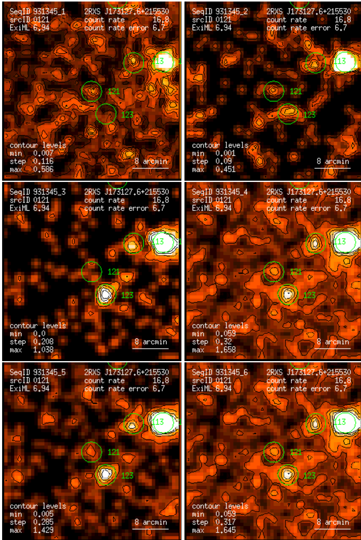
Figure 121: RASS 931345: detection 0121: band rate images, Gaussian filter: (1) PSPC channels 11 – 41, (2) 52 – 90, (3) 91 – 201, (4) 11 – 235, (5) 52 – 201, (6) 11 – 201. Broad band rates in counts/ks. Band rate contour levels in counts/ks/arcmin 2 .
