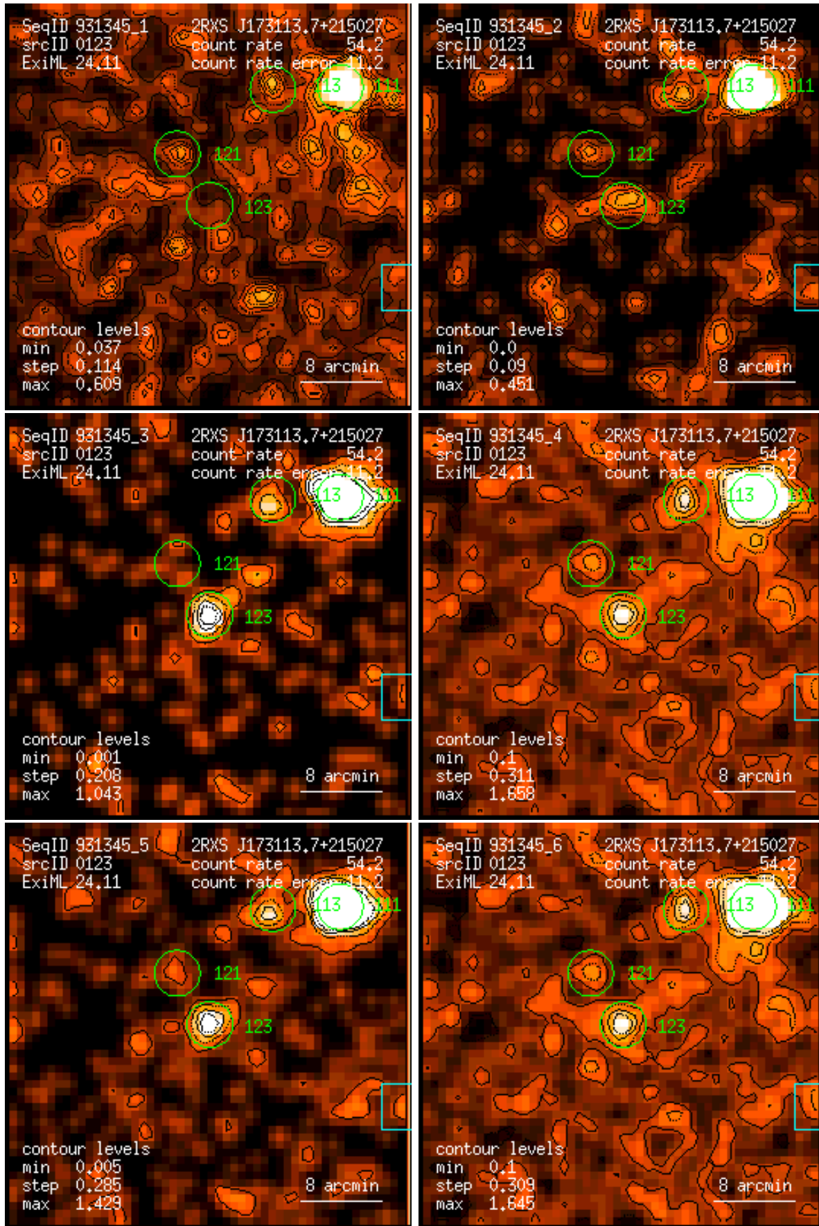
Figure 123: RASS 931345: detection 0123: band rate images, Gaussian filter: (1) PSPC channels 11 – 41, (2) 52 – 90, (3) 91 – 201, (4) 11 – 235, (5) 52 – 201, (6) 11 – 201. Broad band rates in counts/ks. Band rate contour levels in counts/ks/arcmin 2 .
