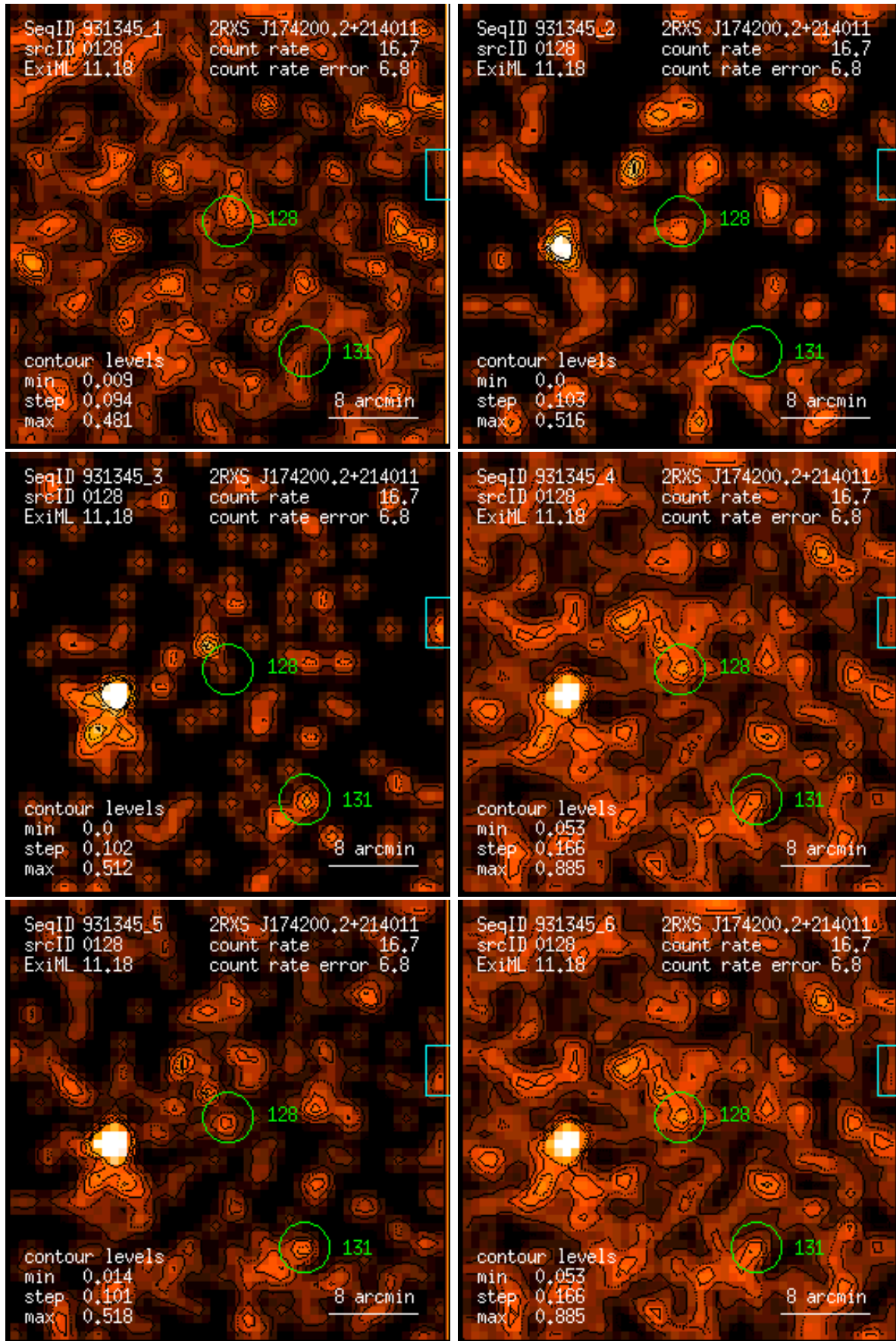
Figure 128: RASS 931345: detection 0128: band rate images, Gaussian filter: (1) PSPC channels 11 – 41, (2) 52 – 90, (3) 91 – 201, (4) 11 – 235, (5) 52 – 201, (6) 11 – 201. Broad band rates in counts/ks. Band rate contour levels in counts/ks/arcmin 2 .
