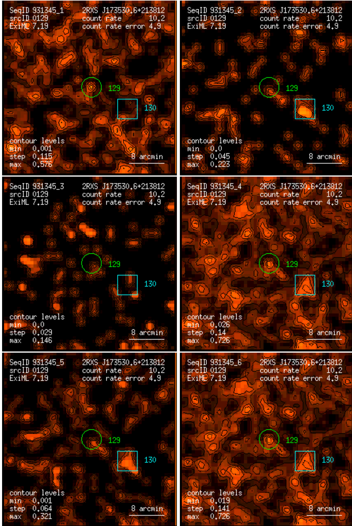
Figure 129: RASS 931345: detection 0129: band rate images, Gaussian filter: (1) PSPC channels 11 – 41, (2) 52 – 90, (3) 91 – 201, (4) 11 – 235, (5) 52 – 201, (6) 11 – 201. Broad band rates in counts/ks. Band rate contour levels in counts/ks/arcmin 2 .
