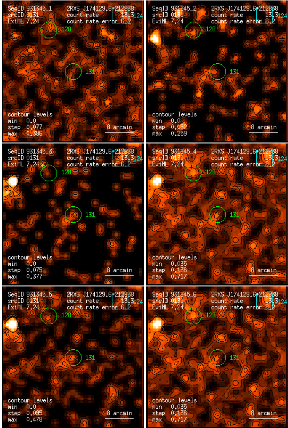
Figure 131: RASS 931345: detection 0131: band rate images, Gaussian filter: (1) PSPC channels 11 – 41, (2) 52 – 90, (3) 91 – 201, (4) 11 – 235, (5) 52 – 201, (6) 11 – 201. Broad band rates in counts/ks. Band rate contour levels in counts/ks/arcmin 2 .
