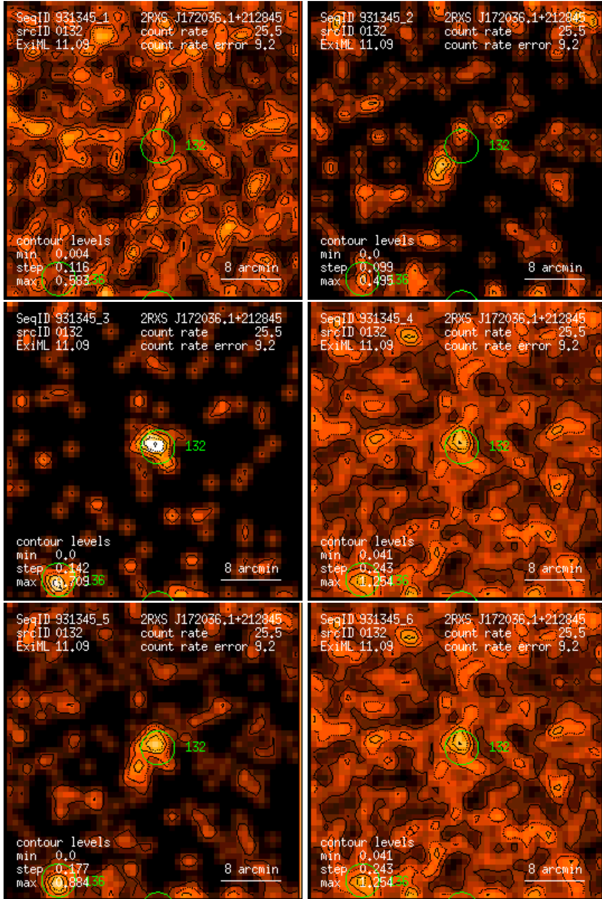
Figure 132: RASS 931345: detection 0132: band rate images, Gaussian filter: (1) PSPC channels 11 – 41, (2) 52 – 90, (3) 91 – 201, (4) 11 – 235, (5) 52 – 201, (6) 11 – 201. Broad band rates in counts/ks. Band rate contour levels in counts/ks/arcmin 2 .
