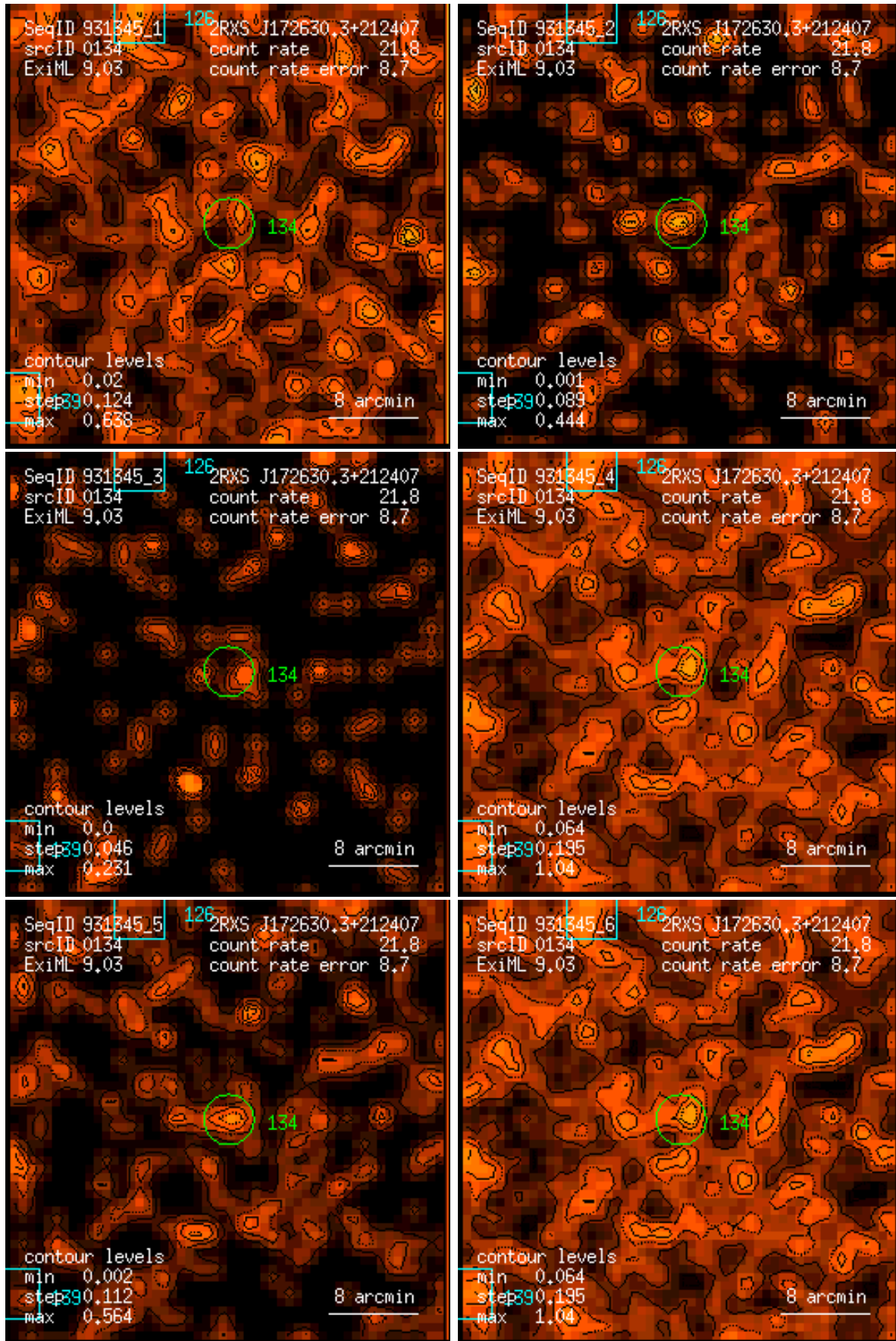
Figure 134: RASS 931345: detection 0134: band rate images, Gaussian filter: (1) PSPC channels 11 – 41, (2) 52 – 90, (3) 91 – 201, (4) 11 – 235, (5) 52 – 201, (6) 11 – 201. Broad band rates in counts/ks. Band rate contour levels in counts/ks/arcmin 2 .
