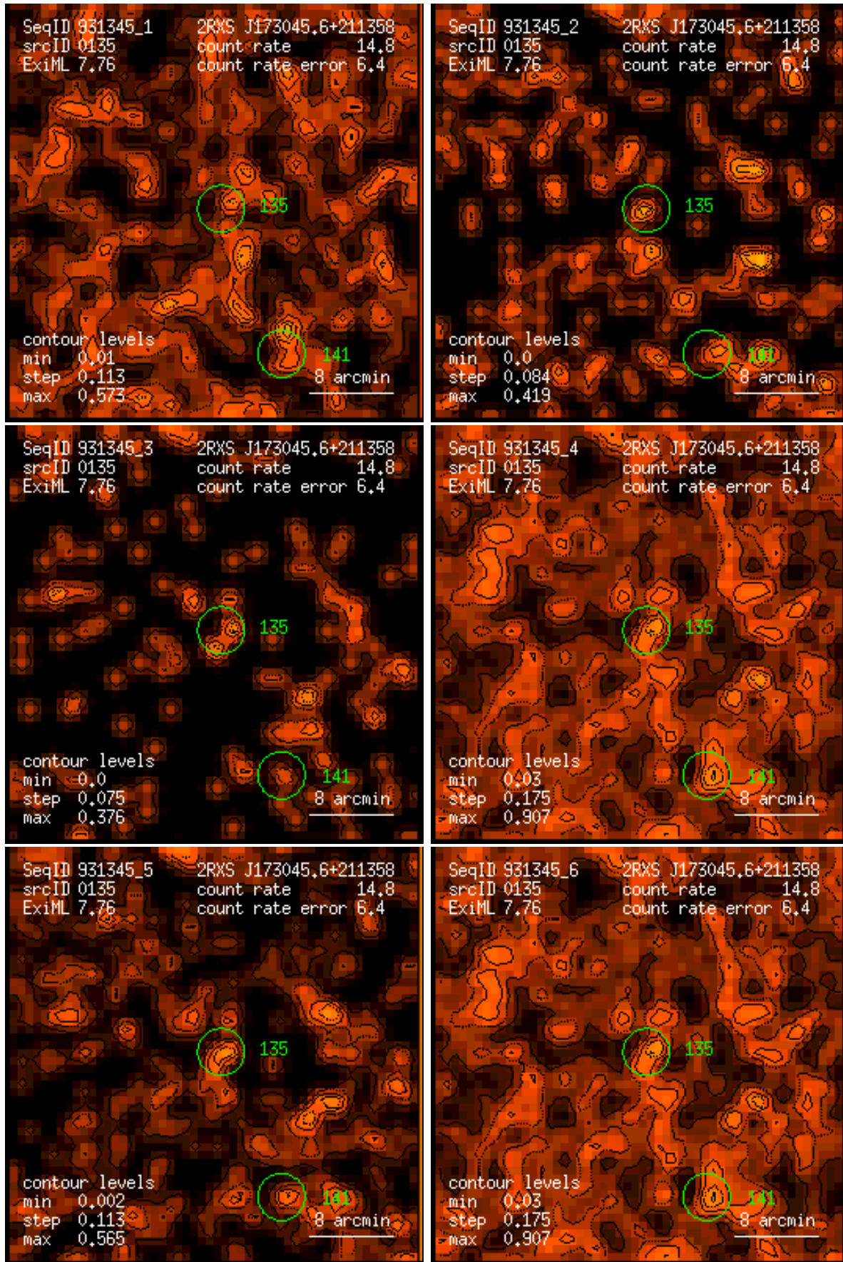
Figure 135: RASS 931345: detection 0135: band rate images, Gaussian filter: (1) PSPC channels 11 – 41, (2) 52 – 90, (3) 91 – 201, (4) 11 – 235, (5) 52 – 201, (6) 11 – 201. Broad band rates in counts/ks. Band rate contour levels in counts/ks/arcmin 2 .
