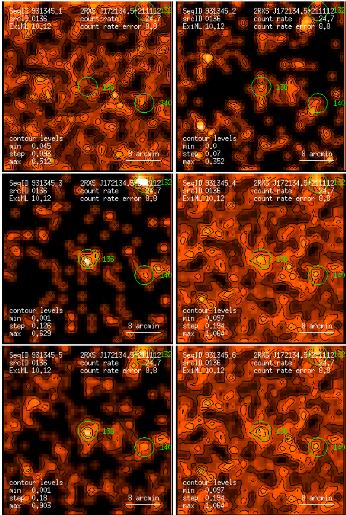
Figure 136: RASS 931345: detection 0136: band rate images, Gaussian filter: (1) PSPC channels 11 – 41, (2) 52 – 90, (3) 91 – 201, (4) 11 – 235, (5) 52 – 201, (6) 11 – 201. Broad band rates in counts/ks. Band rate contour levels in counts/ks/arcmin 2 .
