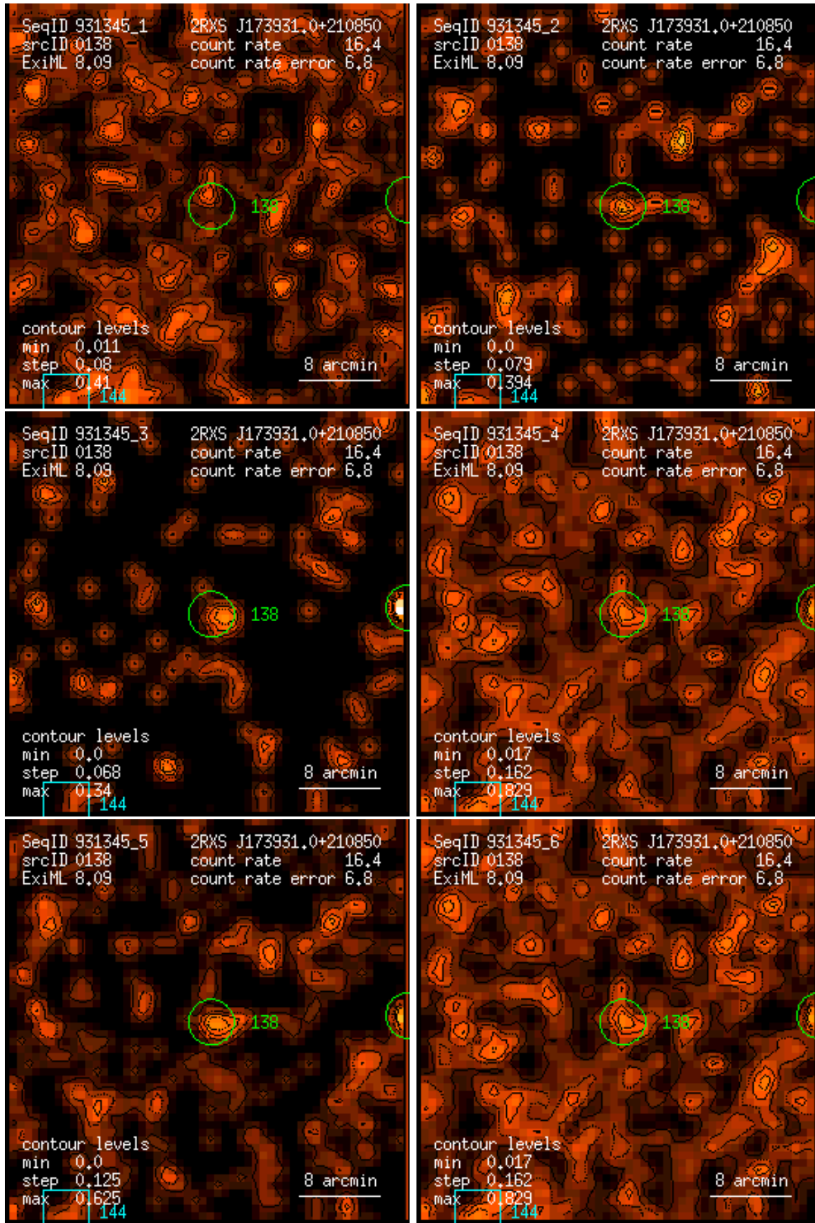
Figure 138: RASS 931345: detection 0138: band rate images, Gaussian filter: (1) PSPC channels 11 – 41, (2) 52 – 90, (3) 91 – 201, (4) 11 – 235, (5) 52 – 201, (6) 11 – 201. Broad band rates in counts/ks. Band rate contour levels in counts/ks/arcmin 2 .
