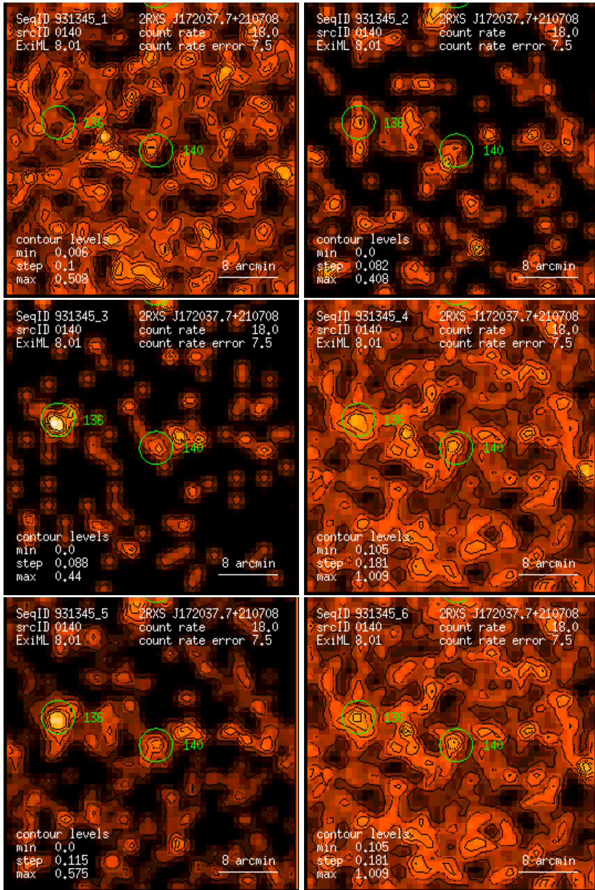
Figure 140: RASS 931345: detection 0140: band rate images, Gaussian filter: (1) PSPC channels 11 – 41, (2) 52 – 90, (3) 91 – 201, (4) 11 – 235, (5) 52 – 201, (6) 11 – 201. Broad band rates in counts/ks. Band rate contour levels in counts/ks/arcmin 2 .
