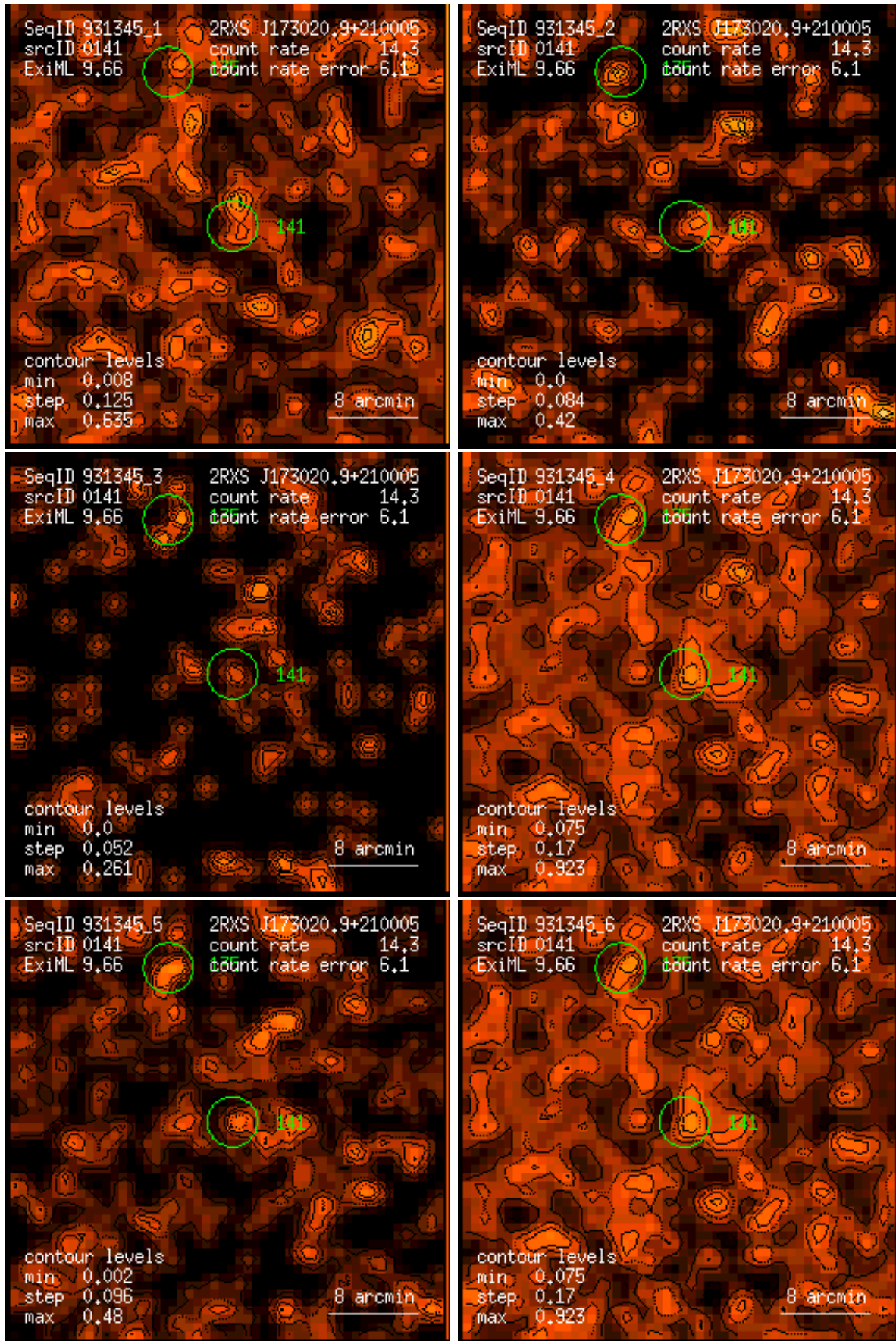
Figure 141: RASS 931345: detection 0141: band rate images, Gaussian filter: (1) PSPC channels 11 – 41, (2) 52 – 90, (3) 91 – 201, (4) 11 – 235, (5) 52 – 201, (6) 11 – 201. Broad band rates in counts/ks. Band rate contour levels in counts/ks/arcmin 2 .
