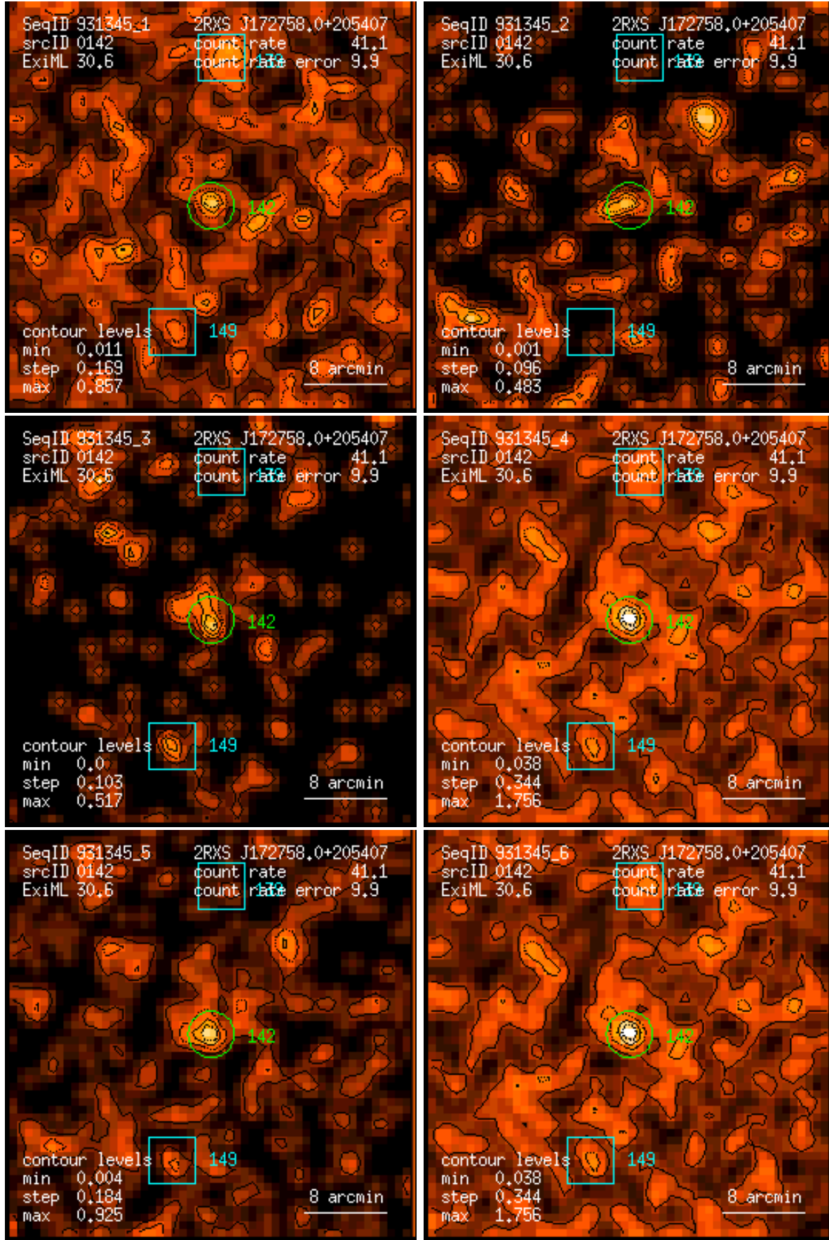
Figure 142: RASS 931345: detection 0142: band rate images, Gaussian filter: (1) PSPC channels 11 – 41, (2) 52 – 90, (3) 91 – 201, (4) 11 – 235, (5) 52 – 201, (6) 11 – 201. Broad band rates in counts/ks. Band rate contour levels in counts/ks/arcmin 2 .
