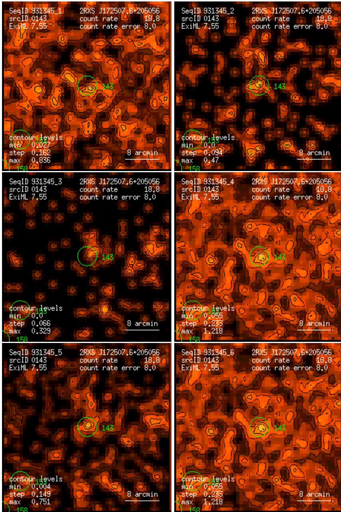
Figure 143: RASS 931345: detection 0143: band rate images, Gaussian filter: (1) PSPC channels 11 – 41, (2) 52 – 90, (3) 91 – 201, (4) 11 – 235, (5) 52 – 201, (6) 11 – 201. Broad band rates in counts/ks. Band rate contour levels in counts/ks/arcmin 2 .
