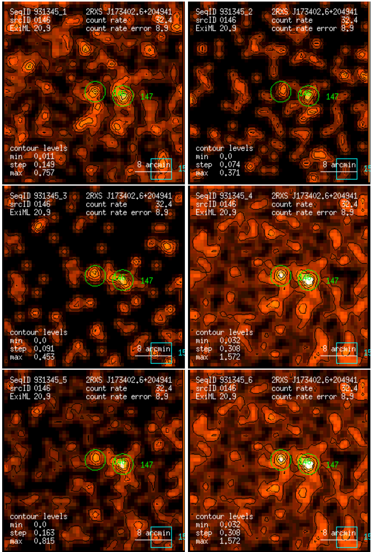
Figure 146: RASS 931345: detection 0146: band rate images, Gaussian filter: (1) PSPC channels 11 – 41, (2) 52 – 90, (3) 91 – 201, (4) 11 – 235, (5) 52 – 201, (6) 11 – 201. Broad band rates in counts/ks. Band rate contour levels in counts/ks/arcmin 2 .
