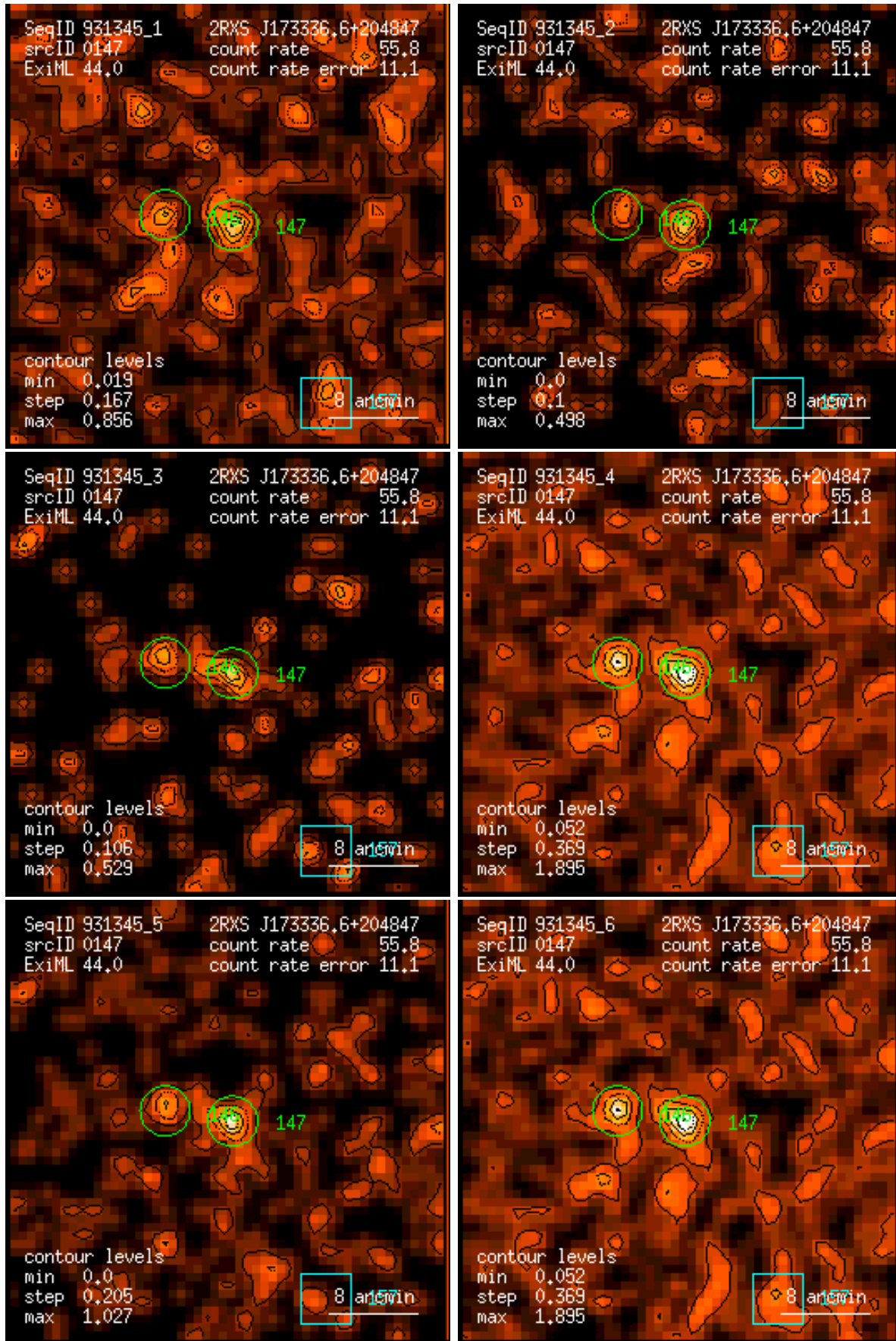
Figure 147: RASS 931345: detection 0147: band rate images, Gaussian filter: (1) PSPC channels 11 – 41, (2) 52 – 90, (3) 91 – 201, (4) 11 – 235, (5) 52 – 201, (6) 11 – 201. Broad band rates in counts/ks. Band rate contour levels in counts/ks/arcmin 2 .
