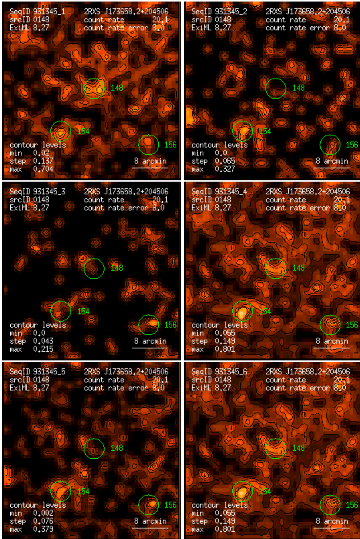
Figure 148: RASS 931345: detection 0148: band rate images, Gaussian filter: (1) PSPC channels 11 – 41, (2) 52 – 90, (3) 91 – 201, (4) 11 – 235, (5) 52 – 201, (6) 11 – 201. Broad band rates in counts/ks. Band rate contour levels in counts/ks/arcmin 2 .
