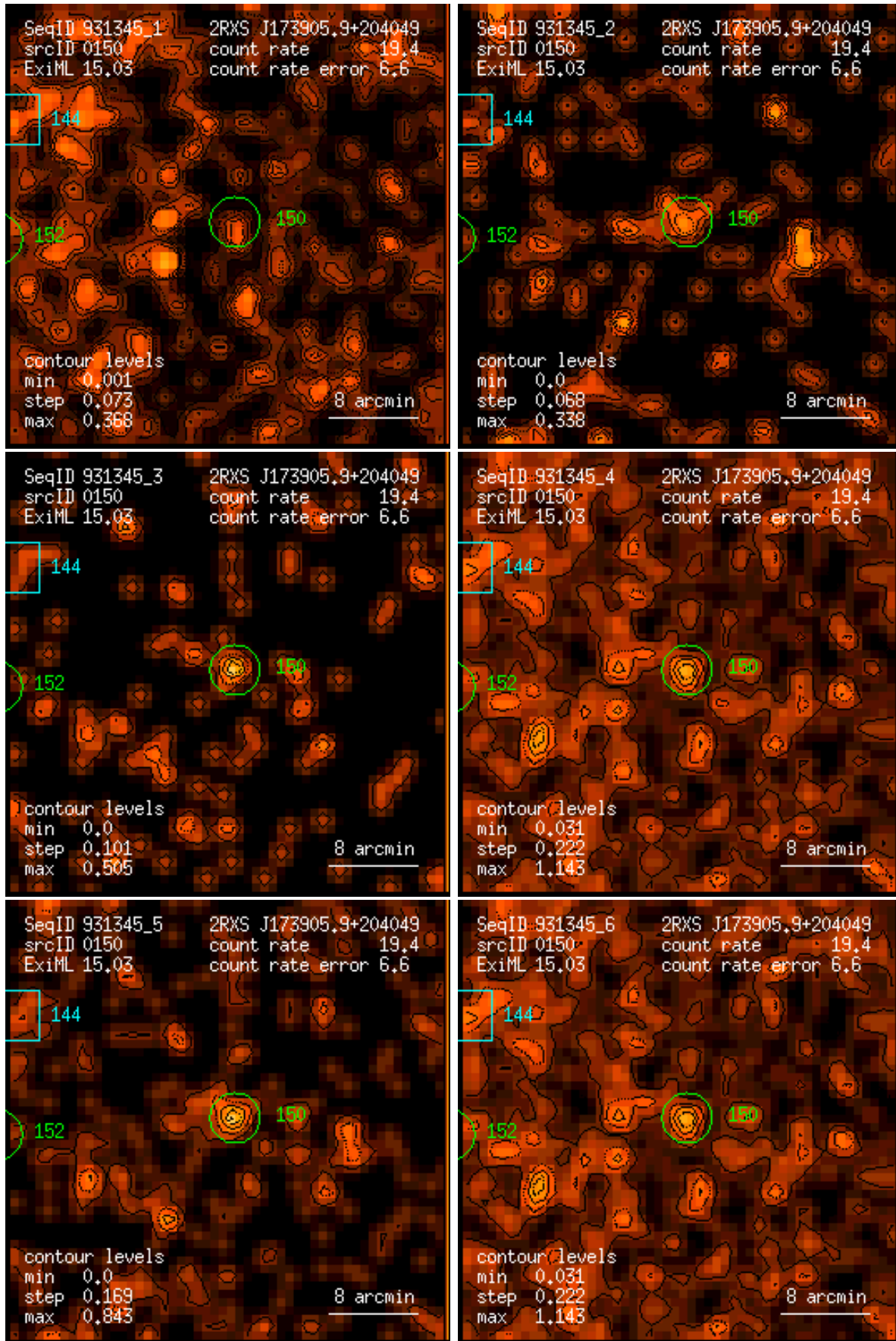
Figure 150: RASS 931345: detection 0150: band rate images, Gaussian filter: (1) PSPC channels 11 – 41, (2) 52 – 90, (3) 91 – 201, (4) 11 – 235, (5) 52 – 201, (6) 11 – 201. Broad band rates in counts/ks. Band rate contour levels in counts/ks/arcmin 2 .
