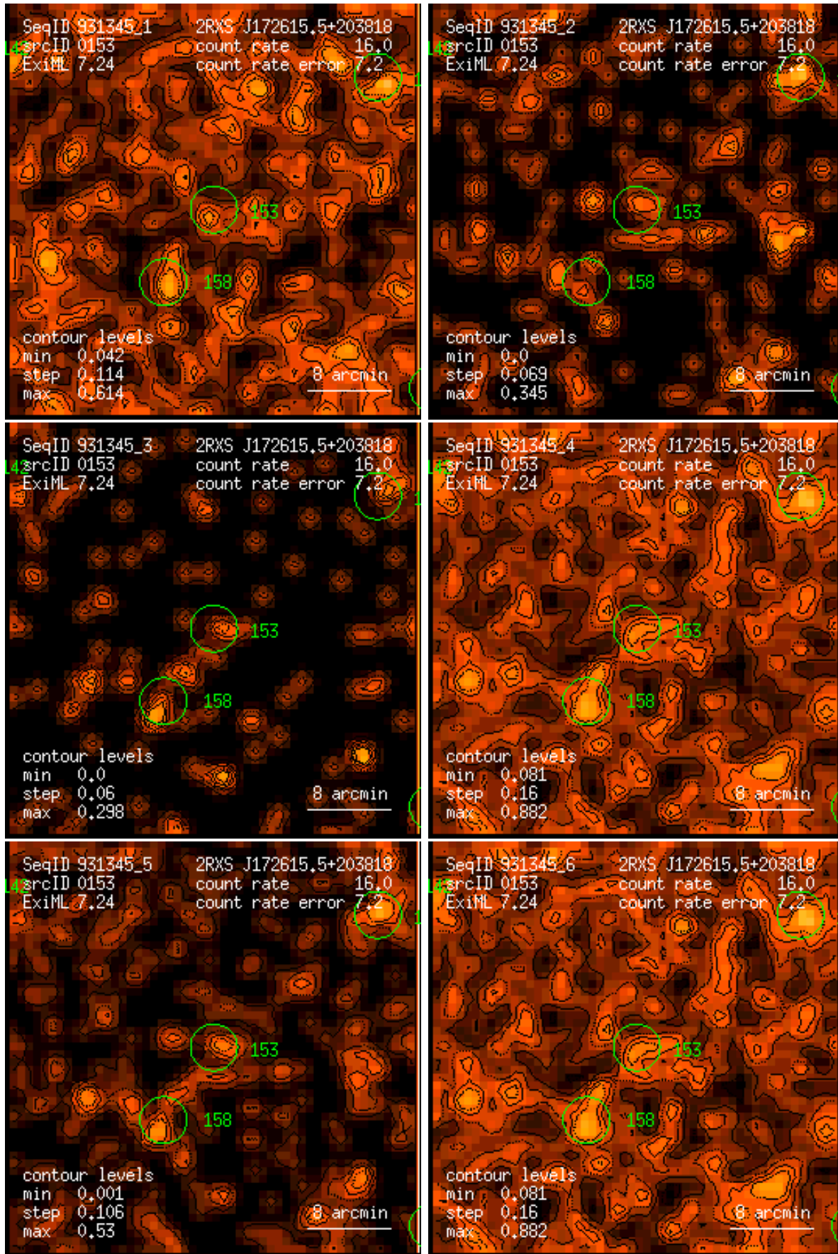
Figure 153: RASS 931345: detection 0153: band rate images, Gaussian filter: (1) PSPC channels 11 – 41, (2) 52 – 90, (3) 91 – 201, (4) 11 – 235, (5) 52 – 201, (6) 11 – 201. Broad band rates in counts/ks. Band rate contour levels in counts/ks/arcmin 2 .
