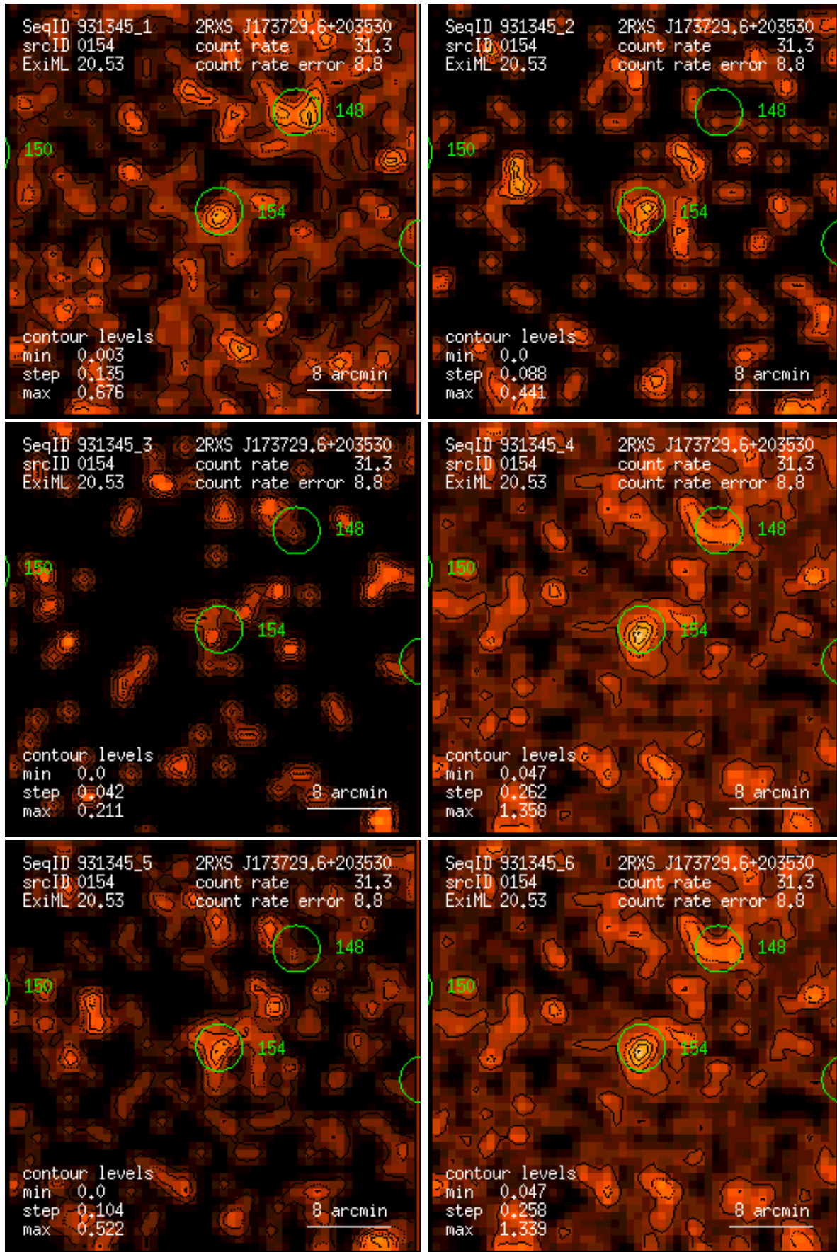
Figure 154: RASS 931345: detection 0154: band rate images, Gaussian filter: (1) PSPC channels 11 – 41, (2) 52 – 90, (3) 91 – 201, (4) 11 – 235, (5) 52 – 201, (6) 11 – 201. Broad band rates in counts/ks. Band rate contour levels in counts/ks/arcmin 2 .
