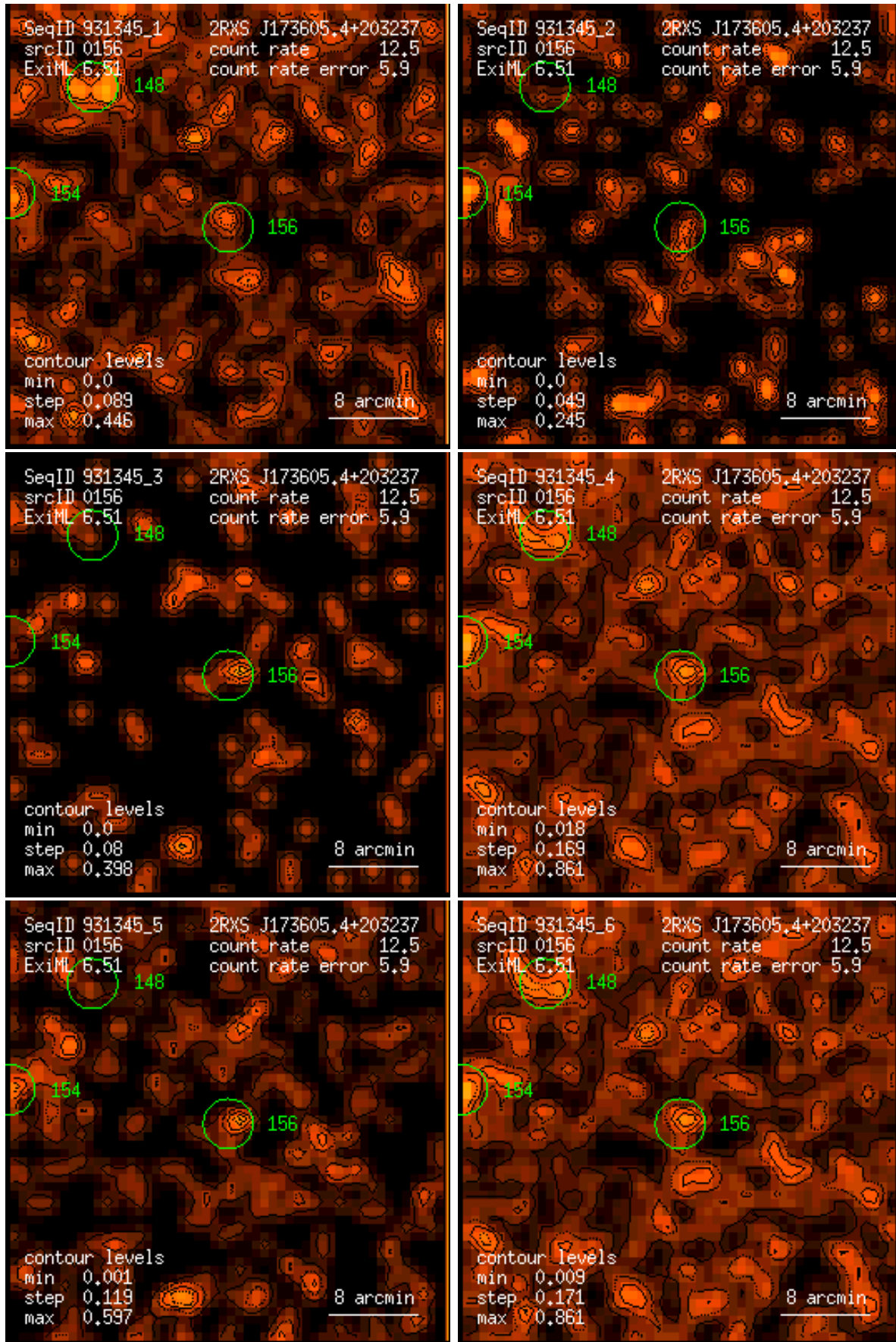
Figure 156: RASS 931345: detection 0156: band rate images, Gaussian filter: (1) PSPC channels 11 – 41, (2) 52 – 90, (3) 91 – 201, (4) 11 – 235, (5) 52 – 201, (6) 11 – 201. Broad band rates in counts/ks. Band rate contour levels in counts/ks/arcmin 2 .
