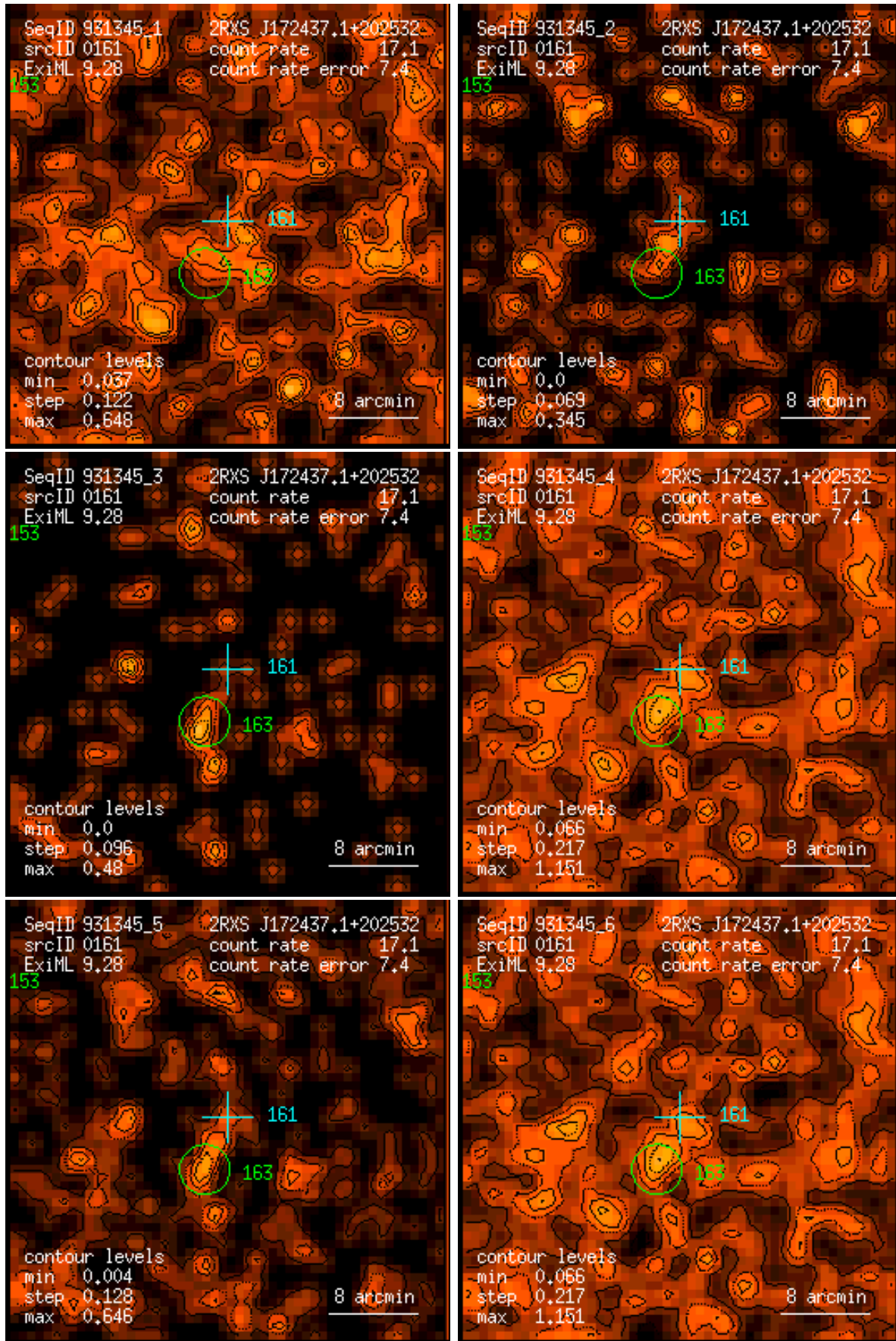
Figure 161: RASS 931345: detection 0161: band rate images, Gaussian filter: (1) PSPC channels 11 – 41, (2) 52 – 90, (3) 91 – 201, (4) 11 – 235, (5) 52 – 201, (6) 11 – 201. Broad band rates in counts/ks. Band rate contour levels in counts/ks/arcmin 2 .
