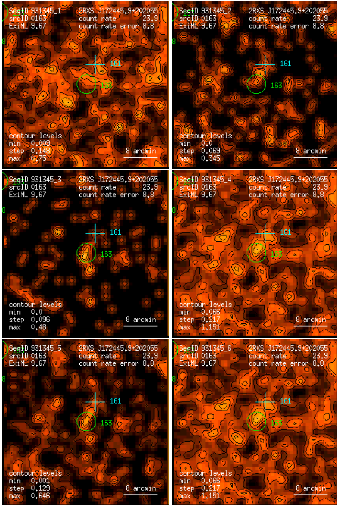
Figure 163: RASS 931345: detection 0163: band rate images, Gaussian filter: (1) PSPC channels 11 – 41, (2) 52 – 90, (3) 91 – 201, (4) 11 – 235, (5) 52 – 201, (6) 11 – 201. Broad band rates in counts/ks. Band rate contour levels in counts/ks/arcmin 2 .
