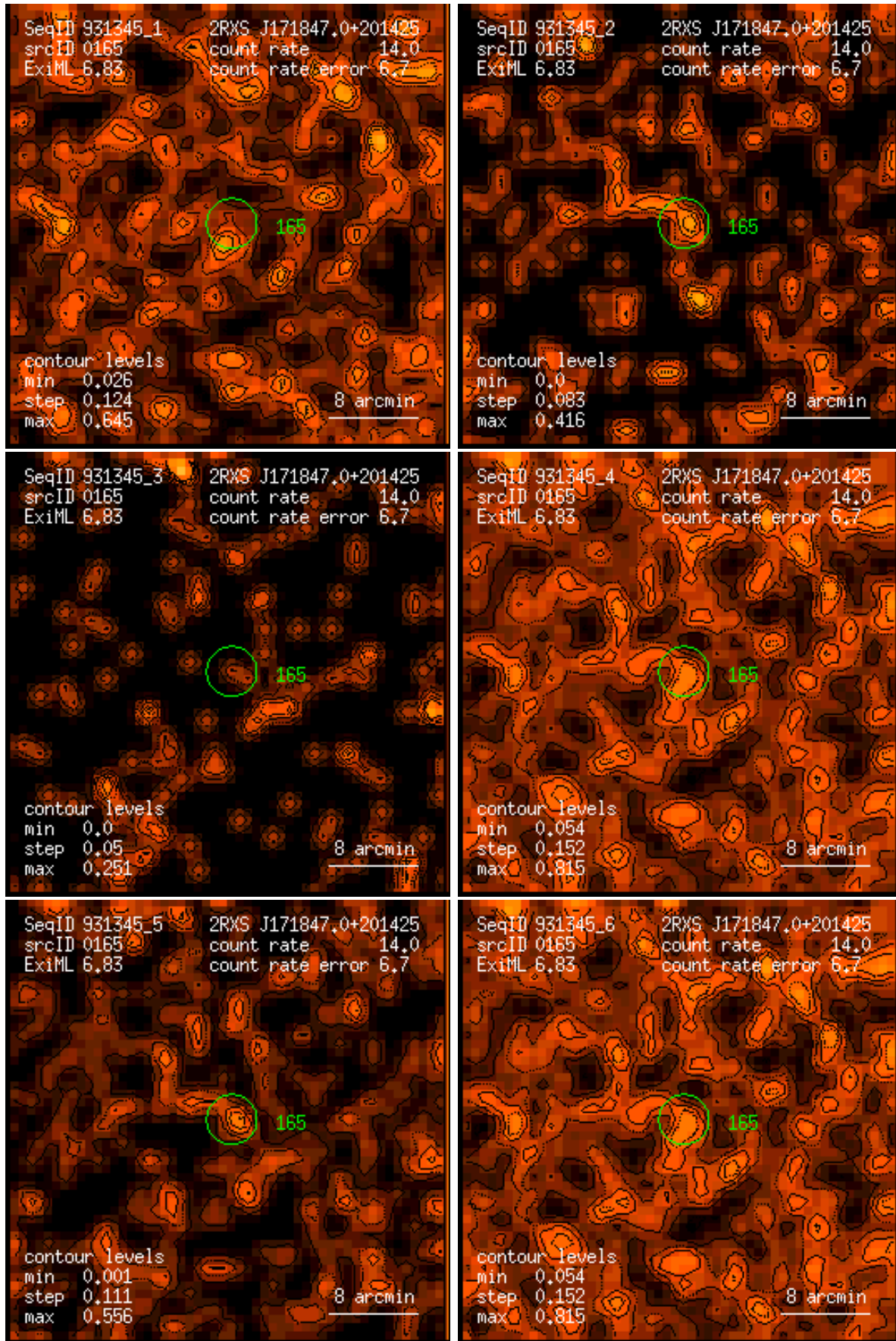
Figure 165: RASS 931345: detection 0165: band rate images, Gaussian filter: (1) PSPC channels 11 – 41, (2) 52 – 90, (3) 91 – 201, (4) 11 – 235, (5) 52 – 201, (6) 11 – 201. Broad band rates in counts/ks. Band rate contour levels in counts/ks/arcmin 2 .
