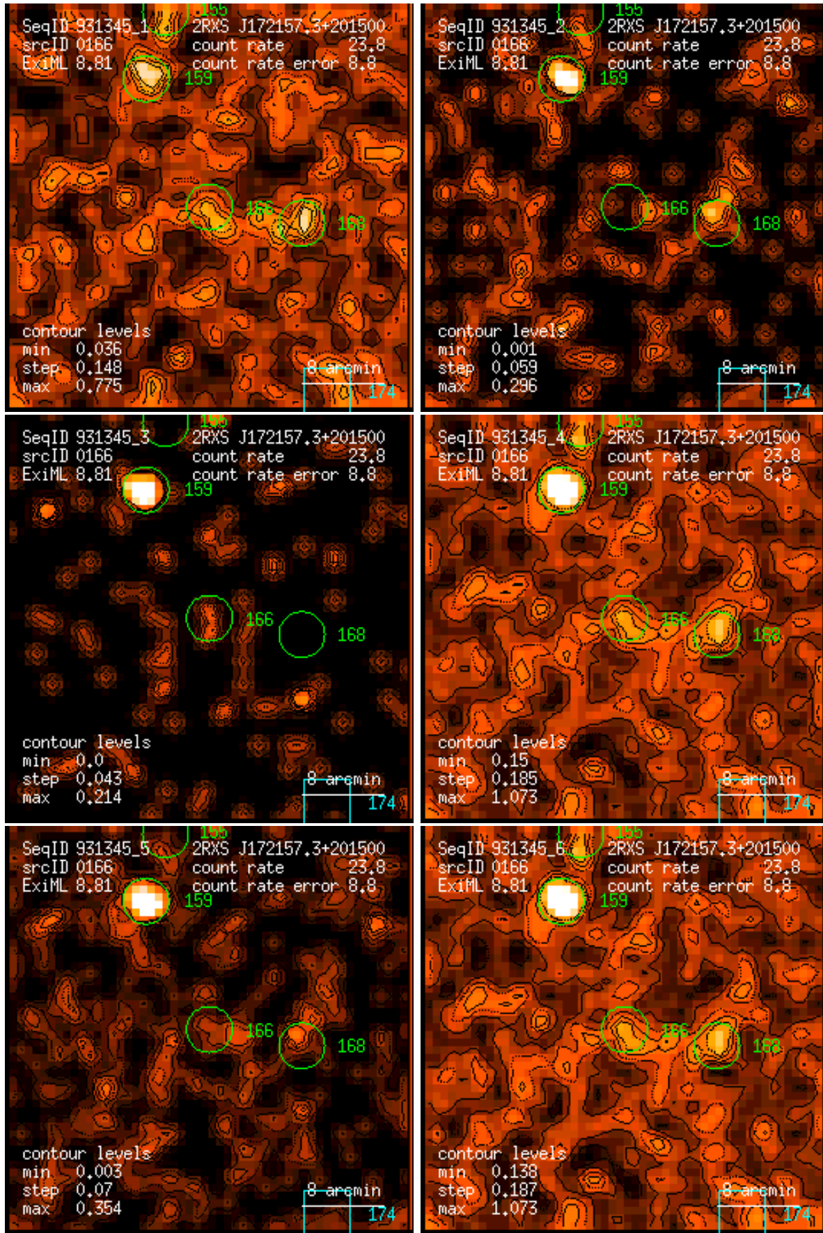
Figure 166: RASS 931345: detection 0166: band rate images, Gaussian filter: (1) PSPC channels 11 – 41, (2) 52 – 90, (3) 91 – 201, (4) 11 – 235, (5) 52 – 201, (6) 11 – 201. Broad band rates in counts/ks. Band rate contour levels in counts/ks/arcmin 2 .
