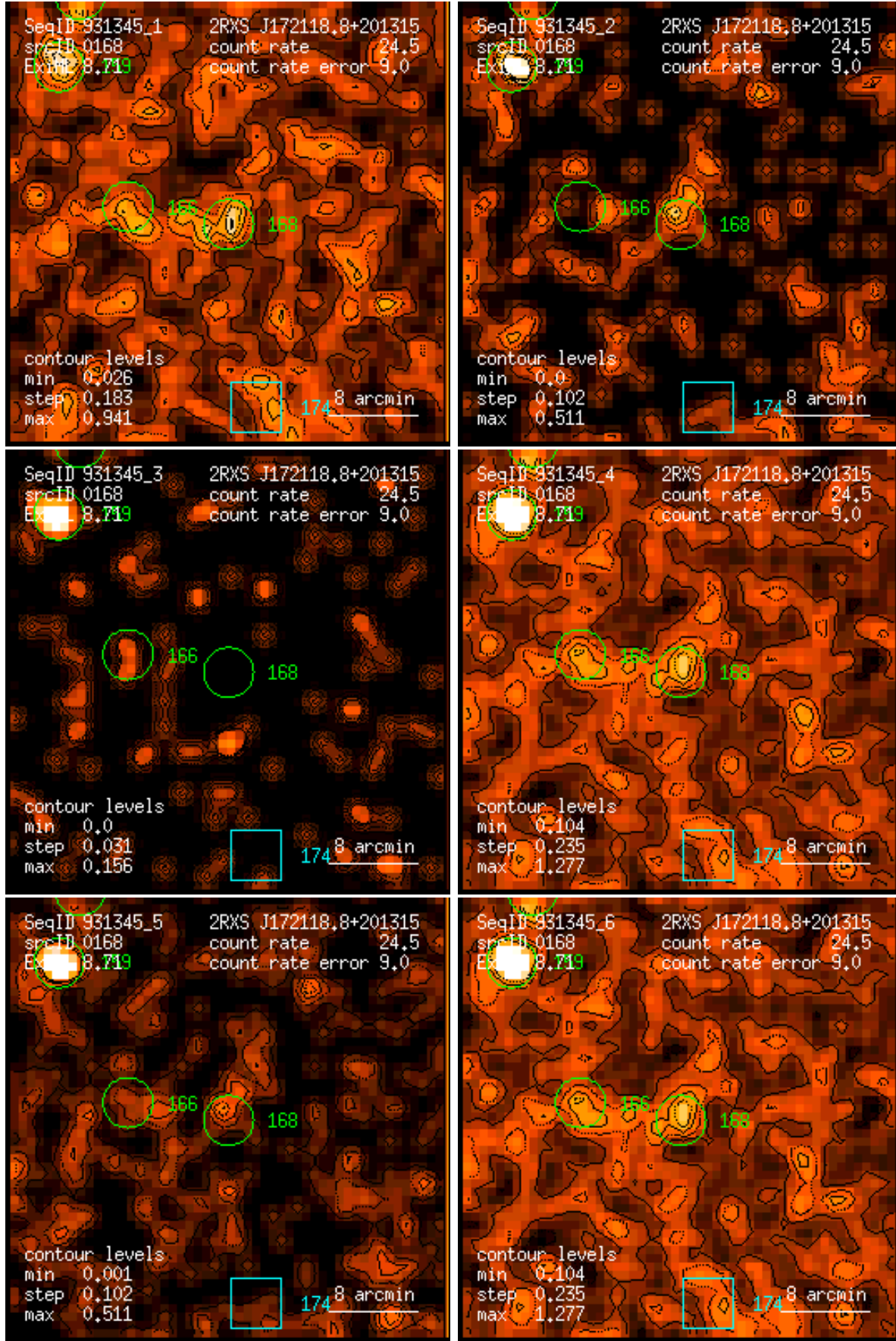
Figure 168: RASS 931345: detection 0168: band rate images, Gaussian filter: (1) PSPC channels 11 – 41, (2) 52 – 90, (3) 91 – 201, (4) 11 – 235, (5) 52 – 201, (6) 11 – 201. Broad band rates in counts/ks. Band rate contour levels in counts/ks/arcmin 2 .
